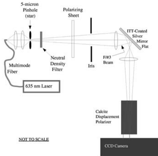
Figure 2. Our experimental setup. A 635-nm laser and 5-micron pinhole simulate our target source. The polarizing sheet ensures linearly polarized incident light for a straightforward analysis. The iris controls unwanted stray light and allows us to increase our F/\# , if desired. The lenses flanking the mirror flat ensure a fast beam (to exacerbate the cross-polarization effect and therefore provide an easily observable aberrated PSF) and an imaged pinhole significantly smaller ( < \lambda / (2 D) ) than resolvable Fraunhofer diffraction pattern features. Our calcite displacement polarizer and CCD camera allow us to record the resultant PSF in orthogonal polarizations.
