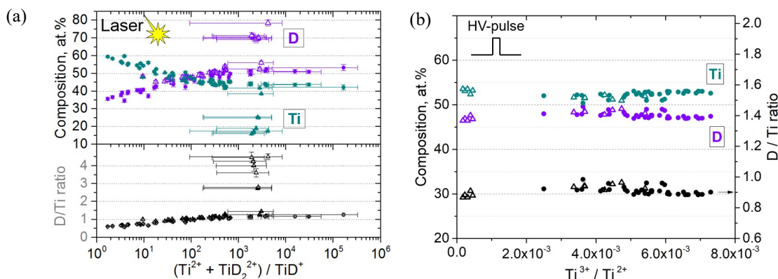
Figure 1. Measured compositions of D and Ti, and the D/Ti ratio as a function of global surface electric field for the measurements with laser pulsing (a) and HV pulsing (b). Data obtained from the LEAP 5000XR are labeled in circles (●) and from the LEAP 5000XS in upper triangles (Δ).
