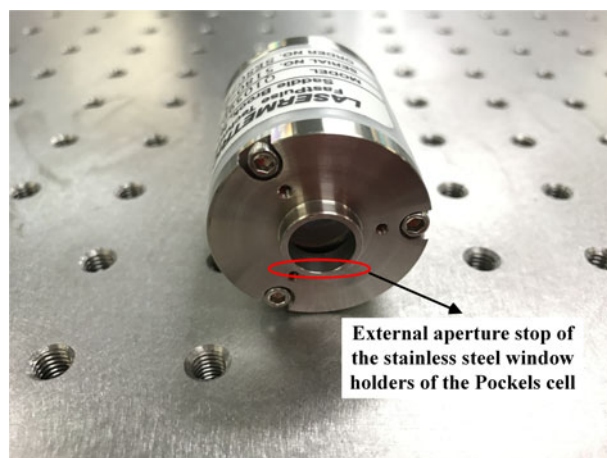
Figure 11. A photo of the PC used in the Regen. The external aperture stop of the stainless steel window holders was marked with a red circle.
