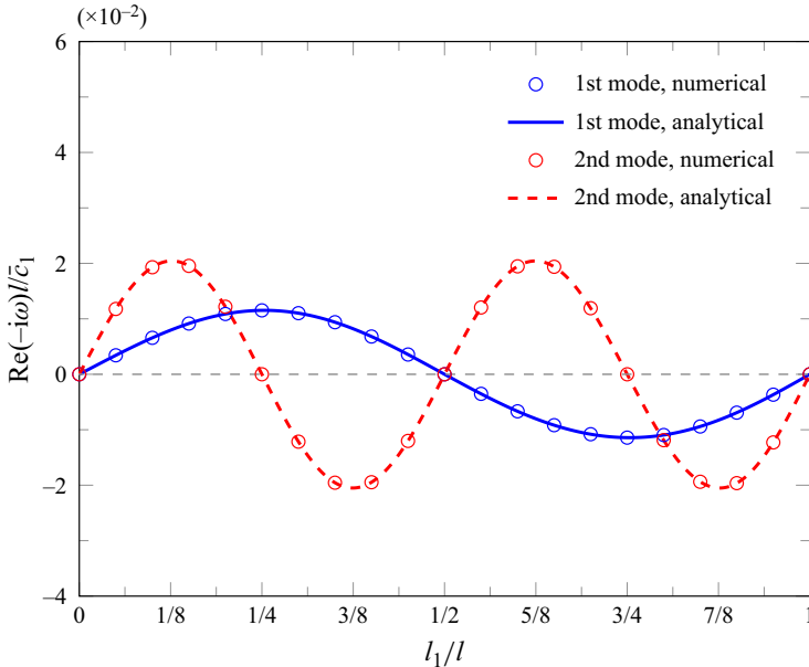
Figure 2. The growth rate obtained from the numerical solution of dispersion relation (2.24) with mean flow \bar{u} = 0 and the unfiltered n - \tau flame model. The results of the first and second eigenmodes are presented.
