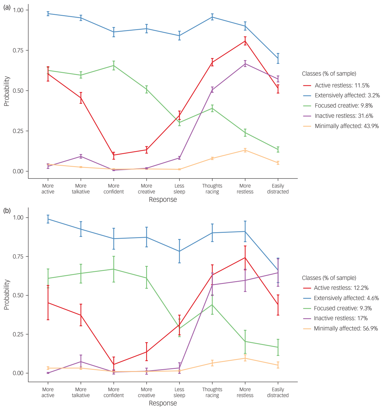
Fig. 1. Conditional probabilities of each response (symptom) in (a) the UK Biobank optimum five-class latent model ( N = 42\,183 ) and (b) the Platform for Research Online to Investigate the Genetics and Cognition in Aging (PROTECT) replication study optimum five-class latent model ( N = 4445 ).
