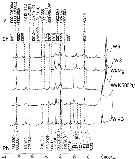
Figure 13. X-ray transmission patterns of the studied samples; \nu = 90^\circ , V = vermiculite 2M_B -VII-meso, Ph = phlogopite-like structure [ 1M_A -I ( 3T_A -IV)] produced after heating of K^+ saturated sample (e.g., W4 K 500°C) or natural phlogopite from Wiry (Wi4B); Ch = chlorite (subfamily C); indices after Bailey (1980); unspecified maxima represent (001) reflections.
