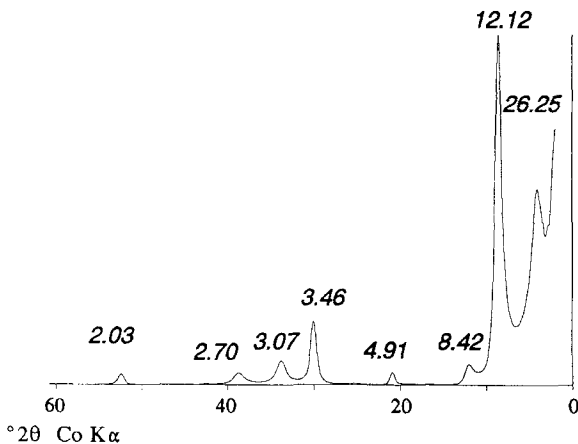
Figure 10. Calculated diffractometer pattern of interstratified trioctahedral mica (0.6)-trioctahedral Mg vermiculite (0.4). R = 1.
