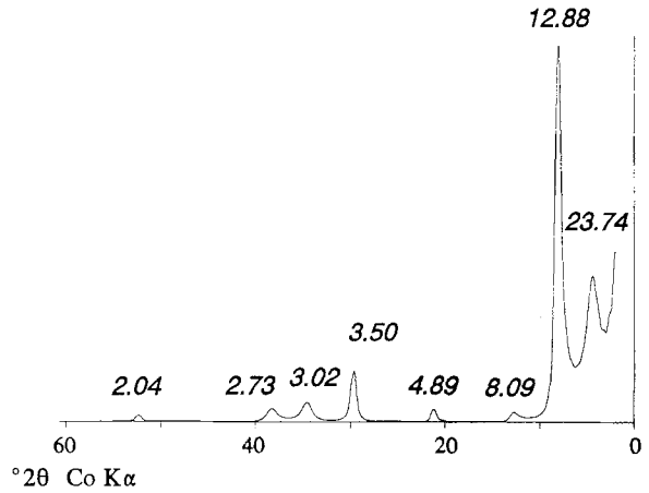
Figure 7. Calculated diffractometer pattern (CoK \alpha ) of interstratified trioctahedral (two water layer) Mg vermiculite (0.6)-trioctahedral mica (0.4) symmetrical distribution of iron. R = 1; d-values correspond to those on 6 (the lower pattern).
