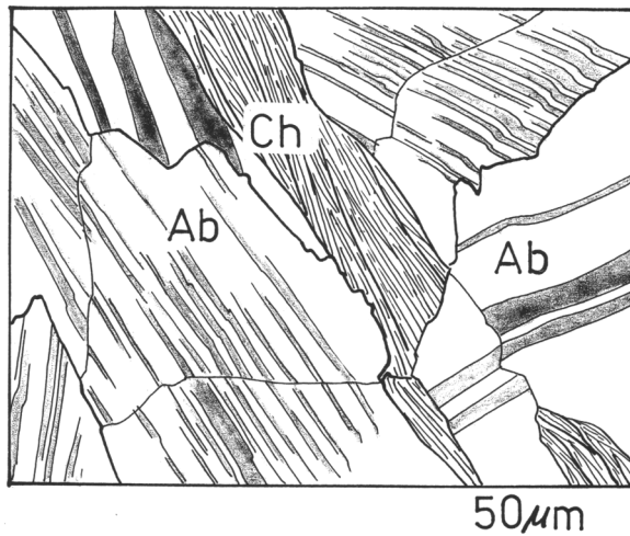
Figure 3. Highly tectonized albite (Ab) pegmatite, with chlorite (Ch) contact schist displaced into the pegmatite fracture, sketch after thin section, sample W106 (contact zone not shown in Figure 2).
