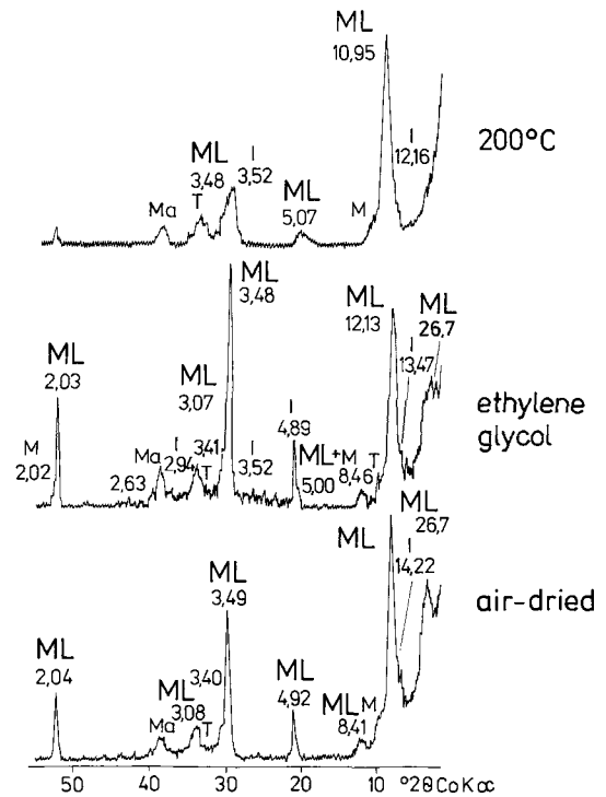
Figure 8. X-ray diffractograms of sample 3-W, reflection method: I = intergrade, ML = mixed layer. For other explanation, see Figure 6.
