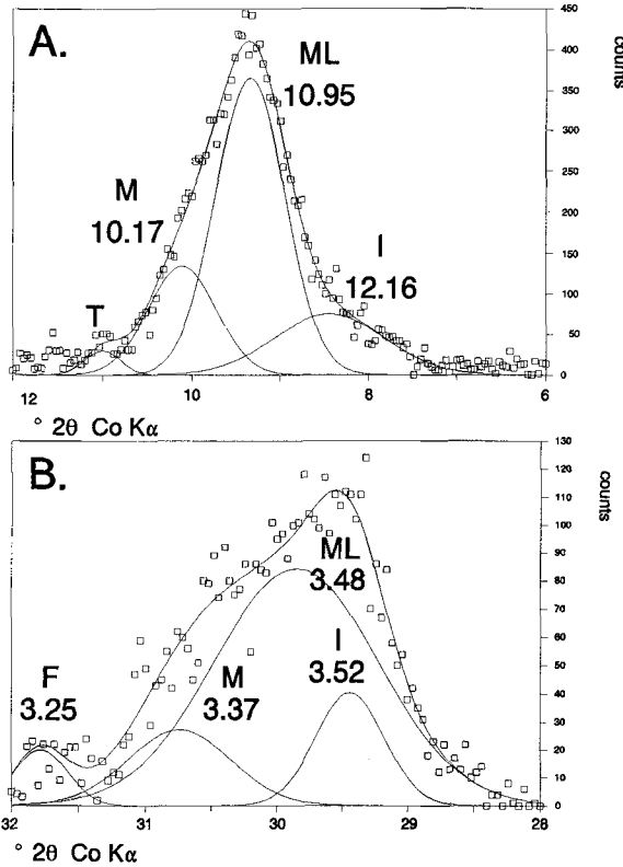
Figure 9. Deconvolution of large diffraction maxima (Figure 6, pattern of sample heated at 200°C in the ranges: A) 7°–11° 2θ, B) 28°–31.5° 2θ. Squares = experimental points, F = K-feldspar, I = intergrade, M = mica, ML = mixed layer, T = talc.
