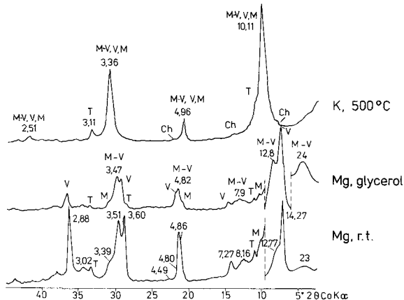
Figure 6. X-ray reflection tracings of sample W4 (4-16 μm): Ch = chlorite, M = mica, M-V = interstratified mica-vermiculite, T = talc, V = vermiculite, r.t. = room temperature. d-values were determined by deconvolution of experimental pattern. Some of them are almost hidden at first glance; their real position often differs from maxima at the tracings.
