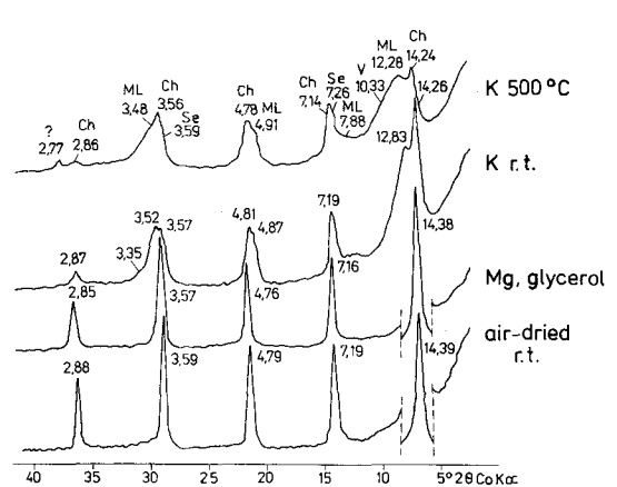
Figure 12. X-ray reflection tracings of sample W9 ( \phi < 0.5 \mu\text{m} ), oriented aggregates. ML = irregularly interstratified chlorite (0.55)-smectite (0.45); Se = serpentine.
