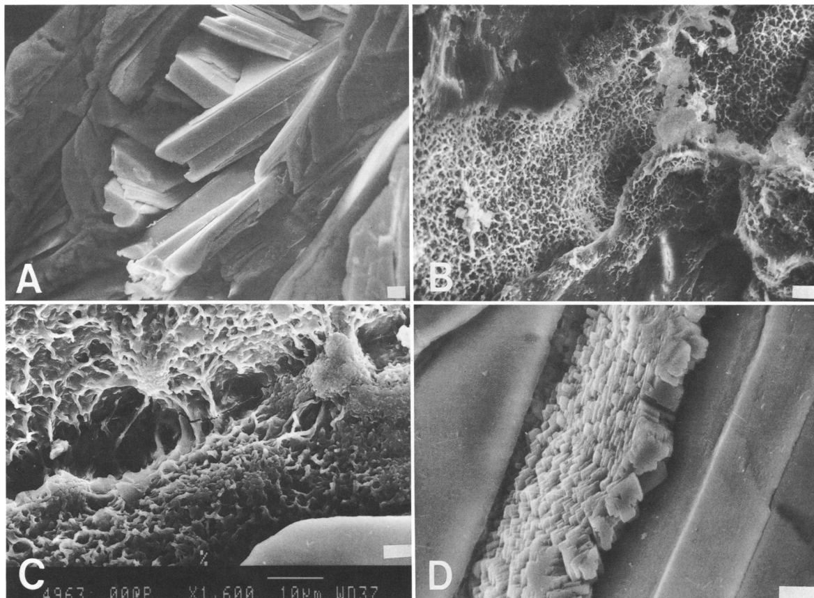
Figure 4. A) Fresh flakes of chlorite in sample W8 after ultrasonic treatment (UST), SEM; B) spongy coatings of a smectite covering large flakes of vermiculite, SEM, sample W3; C) blistering mica surface (1), large and fresh flake of vermiculite (2) and relic spongy aggregates of smectite (3), sample W1 after UST, SEM; D) rhomboidal small magnesite crystal in between large mica flakes, sample W15D after UST, SEM. Bar on SEM photographs represents 5 \mu\text{m} .
