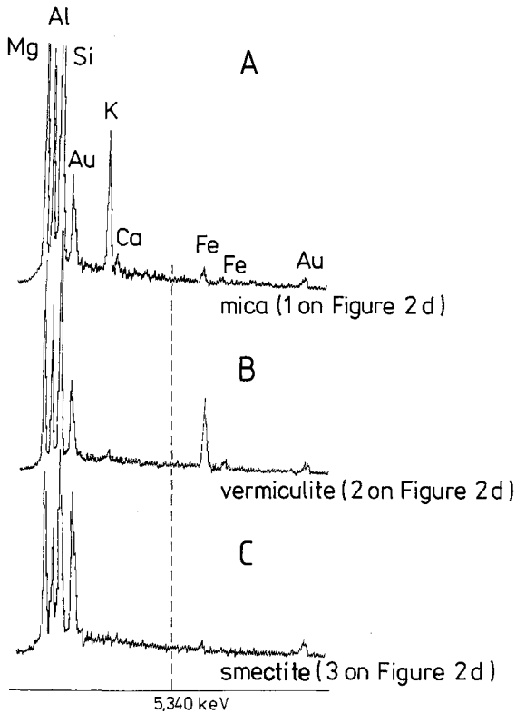
Figure 5. Energy dispersive X-ray spectra: A) blistering surfaces of mica, B) fresh flakes of vermiculite, C) relic smectite coatings in fissure (sample W1 after UST). Au = covering medium.
