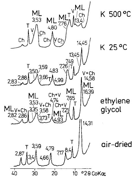
Figure 11. X-ray reflection tracings of sample W7 ( \phi < 0.5 \mu\text{m} ), oriented aggregates, positions of overlapped peaks were determined by deconvolution of experimental pattern (some of them are almost completely hidden at first glance). ML = tri-component interstratified mineral chlorite (0.4)-swelling chlorite (0.35)-smectite (0.25). For explanation see text.
