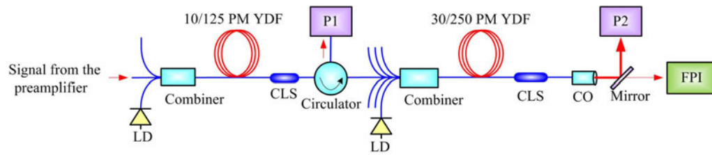
Figure 4. Experimental setup of the LMA fiber amplifier. LD, laser diode; FPI, Fabry–Perot interferometer; P1, P2, power meter; PM YDF, polarization-maintained Yb-doped fiber; CLS, cladding laser stripper; CO, collimator.
