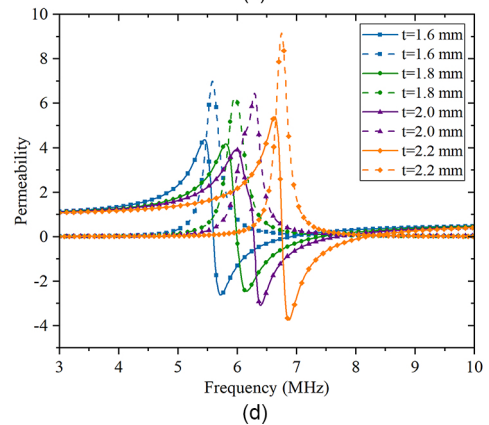
Figure 5. Effective permeability of the MM with different structure parameter variation: (a) turn of spiral N , (b) line width of spiral w , (c) line spacing of spiral s , and (d) thickness of substrate t .
