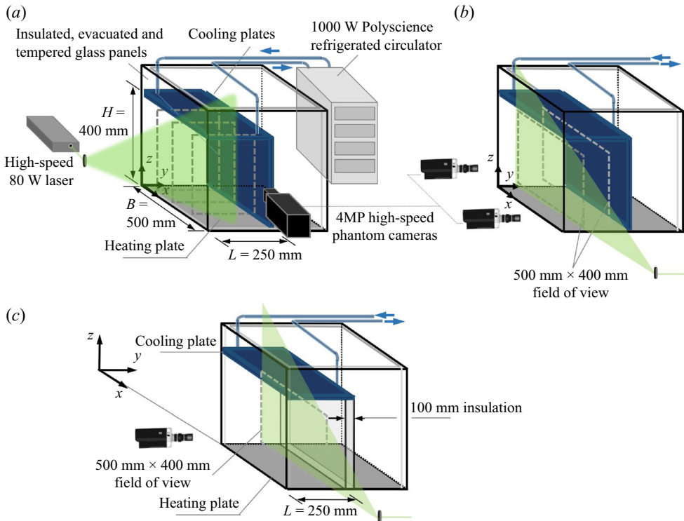
Figure 1. Basic schematic of the experimental set-ups with the large tank illustrating the case with single sidewall cooling with (a) three field of views (FOVs) in the y-z planes at x/B = 1/4, 1/2 and 3/4 and (b) two FOVs in the x-z planes at y/L = 1/3 and 2/3 . (c) Standard RB configuration (no sidewall cooling) showing an x-z FOV plane at y/L = 1/2 . A similar set-up was studied with a smaller tank of half the size; see Appendix A .
