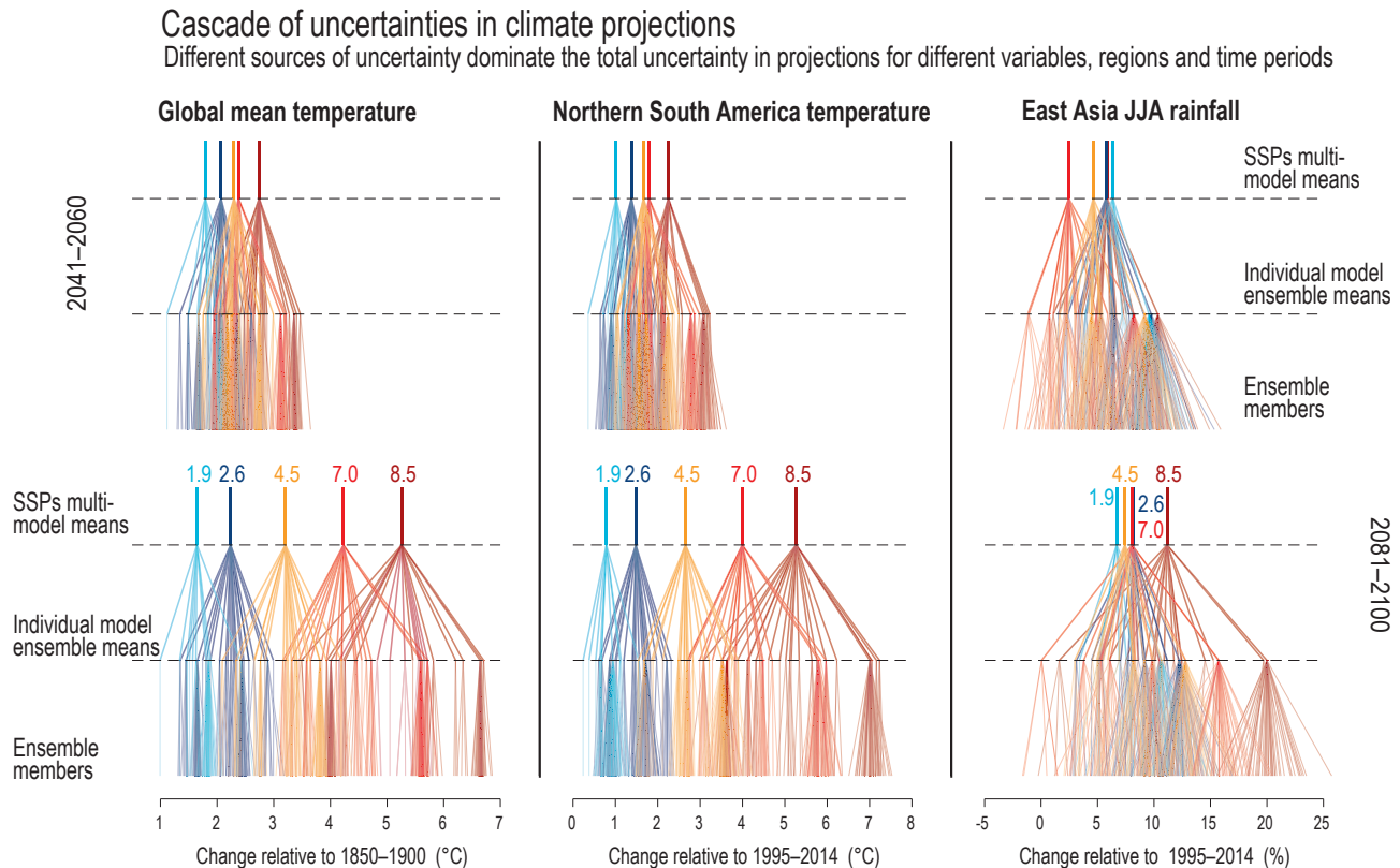
Figure 1.15 | The ‘cascade of uncertainties’ in CMIP6 projections. Changes in: GSAT (left); Northern South America temperature (middle); and East Asia summer (June–July–August, JJA) precipitation (right). These are shown for two time periods: 2041–2060 (top) and 2081–2100 (bottom). The SSP–radiative forcing combination is indicated at the top of each cascade at the value of the multi-model mean for each scenario. This branches downwards to show the ensemble mean for each model, and further branches into the individual ensemble members, although often only a single member is available. These diagrams highlight the relative importance of different sources of uncertainty in climate projections, which varies for different time periods, regions and climate variables. See Section 1.4.5 for the definition of the regions used. Further details on data sources and processing are available in the chapter data table (Table 1.SM.1).
