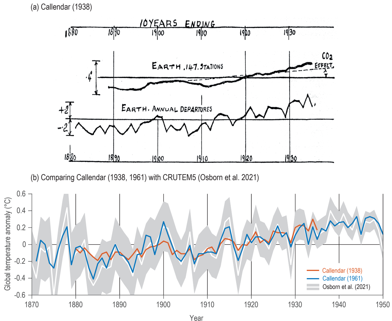
Figure 1.8 | G.S. Callendar’s estimates of global land temperature variations and their possible causes. (a) The original figure from Callendar (1938), using measurements from 147 surface stations for 1880–1935, showing: (top) ten-year moving departures from the mean of 1901–1930 (°C), with the dashed line representing his estimate of the ‘CO 2 effect’ on temperature rise, and (bottom) annual departures from the 1901–1930 mean (°C). (b) Comparing the estimates of global land (60°S–60°N) temperatures tabulated in Callendar (1938, 1961) with a modern reconstruction (CRUTEM5, Osborn et al., 2021) for the same period, following Hawkins and Jones (2013). Further details on data sources and processing are available in the chapter data table (Table 1.SM.1).
