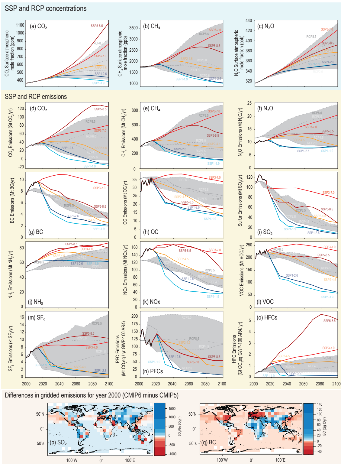
Cross-Chapter Box 1.4, Figure 2 | Comparison between the Shared Socio-economic Pathways (SSP) scenarios and the Representative Concentration Pathway (RCP) scenarios in terms of their \text{CO}_2 , \text{CH}_4 and \text{N}_2\text{O} atmospheric concentrations (a–c), and their global emissions of \text{CO}_2 , \text{CH}_4 , \text{N}_2\text{O} , black carbon (BC), organic carbon (OC), sulphur dioxide ( \text{SO}_2 ), ammonia ( \text{NH}_3 ), nitrogen oxides ( \text{NO}_x ), volatile organic compounds (VOC), sulphur hexafluoride ( \text{SF}_6 ), perfluorocarbons (PFCs), and hydrofluorocarbons (HFCs) (d–o).
