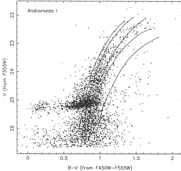
Figure 1. The V , (B - V) color-magnitude diagram for the M31 dSph companion And I from Da Costa et al. (1996). Note the dominance of red horizontal branch (HB) stars though blue HB and RR Lyrae variables are also present. The giant branches of the standard Galactic globular clusters M68 ( [\text{Fe}/\text{H}] = -2.09 ), M55 ( -1.82 ), NGC 6752 ( -1.54 ), NGC 362 ( -1.28 ) and 47 Tuc ( -0.71 ) are superposed assuming (m - M)_V = 24.68 and E(B - V) = 0.04 for And I, together with an additional 0.05 mag redward shift to improve the quality of the overall fit.
