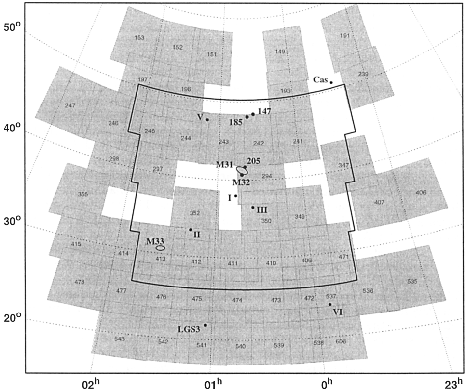
Figure 2. Map of the region of sky around M31 surveyed for low surface brightness dwarf galaxies by Armandroff et al. (1998a, 1999b), showing the POSS-II plates that have been searched. The area surveyed by van den Bergh (1972, 1974) is outlined in bold. M31, its known neighbors, and the new M31 dSphs And V, And VI and Cas are labeled.
