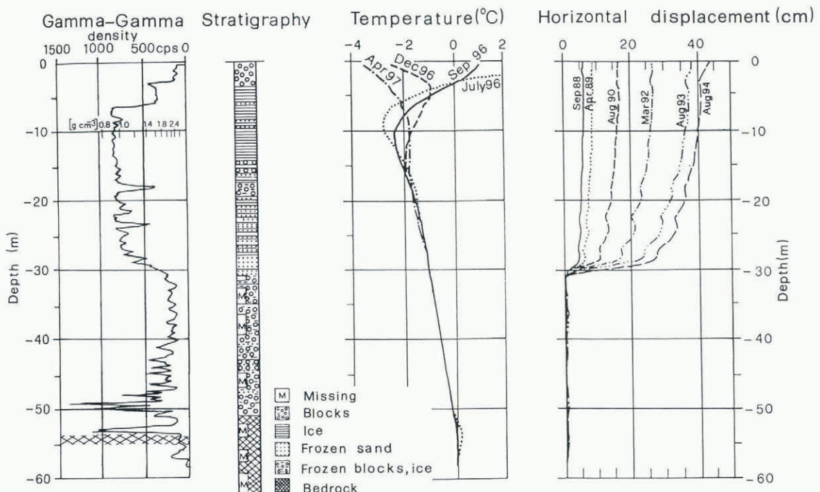
Fig. 4. Principal results from core analyses and borehole measurements at the active rock glacier Murtèl–Corvatsch. Underneath the 3 m thick active layer with coarse blocks, the density log ( \gamma-\gamma ) and the stratigraphy show two main layers: (1) massive ice (90–100% ice content by volume) with thin layers of ice-rich sand down to 28 m, and (2) coarse blocks with ice-filled pores but almost completely without fine rock particles down to bedrock at about 57 m depth. Three-quarters of the total horizontal displacement ( 6\text{ cm a}^{-1} at the surface) takes place within a pronounced shear horizon in the transition zone between the two layers at 28–30 m depth as revealed by the borehole deformation. The upper (strongly supersaturated) layer undergoing steady-state creep thereby overrides the non-deforming (structured) lower layer. Seasonal temperature variations are well developed within approximately the uppermost 20 m, and mean annual permafrost temperature at the permafrost table (3 m depth) is estimated at -2.5^\circ to -3^\circ\text{C} .
