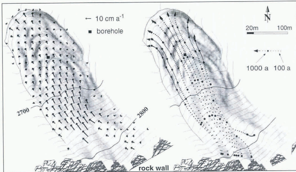
Fig. 3. Surface velocities of rock glacier Murtèl over the period 1986–96, determined by computer-aided photogrammetry (left), and trajectories/surface ages computed from this velocity field (right).
