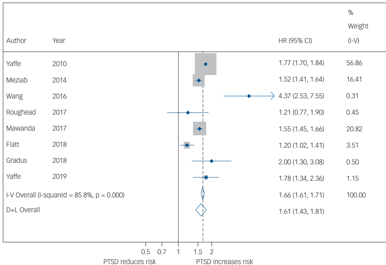
Fig. 2 Meta-analysis of hazard ratios of post-traumatic stress disorder (PTSD) compared with no PTSD on risk of dementia.
