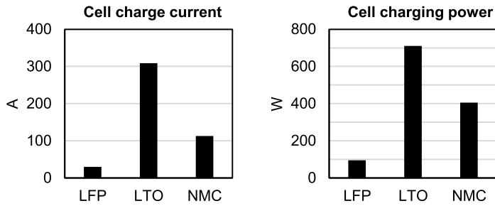
Figure 5. Cell charge current and cell charging power for different cell types.
