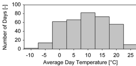
Figure 11. Long-term average yearly temperature distribution for Berlin, generated from Bundesinstitut für Bau-, Stadt- und Raumforschung (2013).
