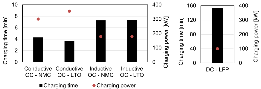
Figure 17. Charging time and actual charging power of the different bus system designs under winter conditions.
