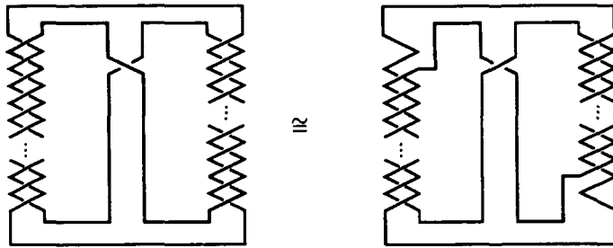
Figure 2: An alternating diagram of L(q, -1, r) .
