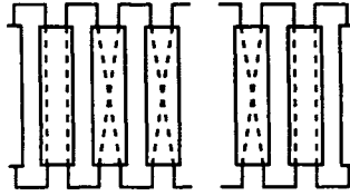
Figure 7: Boundary orientation of L(p_1, p_2, \dots, p_n) .
