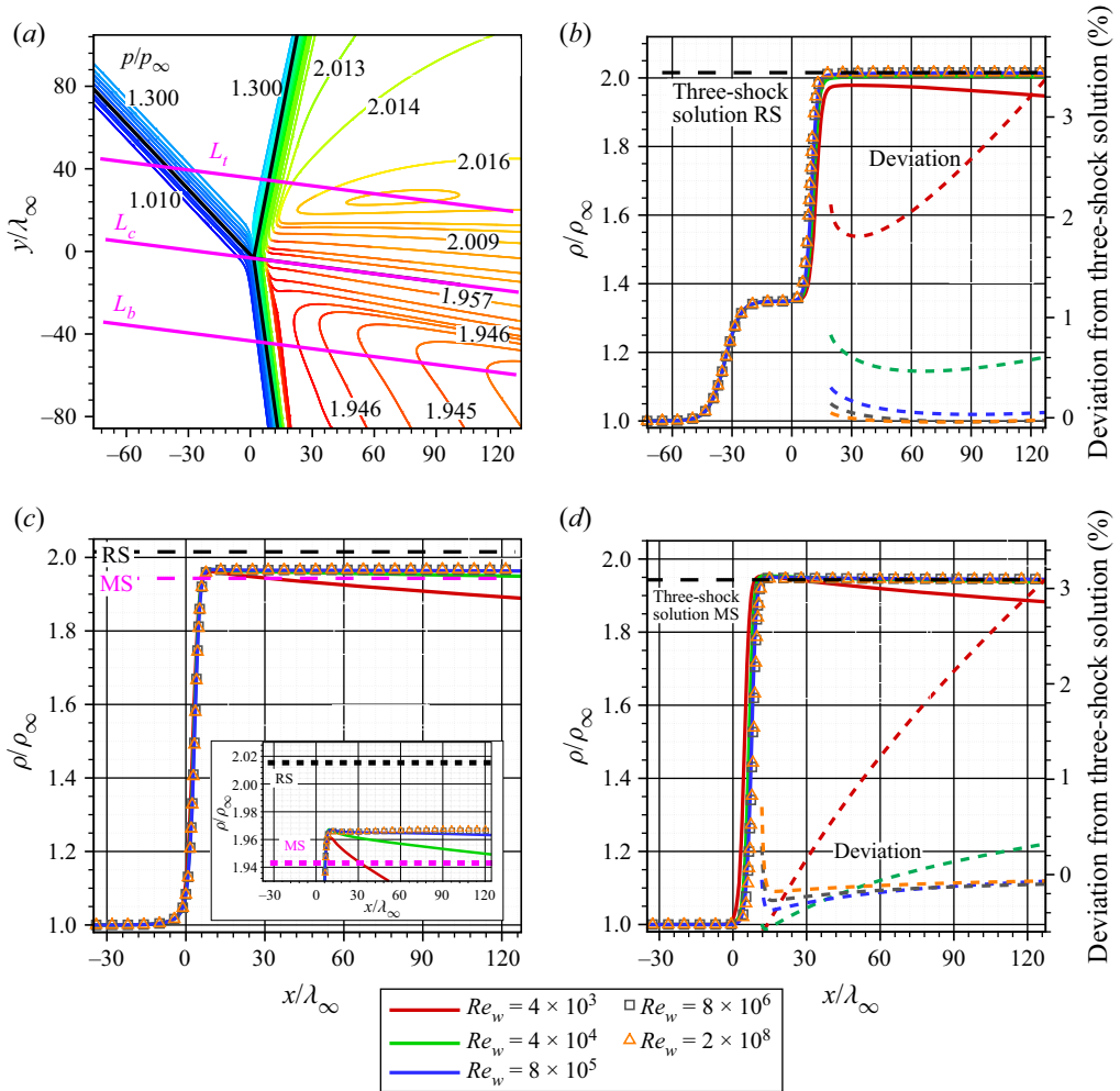
Figure 17. Density contours and distributions at various Re_w . (a) Density contours at Re_w = 2 \times 10^8 . The black solid lines show the three-shock solution. Lines L_t , L_c and L_b are parallel to the slip line of the three-shock solution. (b–d) Density distributions at various Re_w along lines (b) L_t , (c) L_c , and (d) L_b . Lines labelled ‘Three-shock solution RS’, ‘RS’ and ‘Three-shock solution MS’, ‘MS’ show the density according to the three-shock solution behind the RS and MS, respectively. The dashed curves, showing the deviation from the three-shock solution, are labelled ‘Deviation’.
