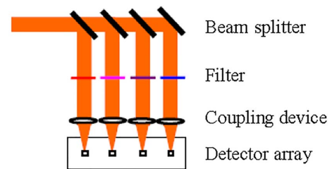
Figure 3. Schematic of a multi-channel THz-diagnostic system based on a direct detector array.
