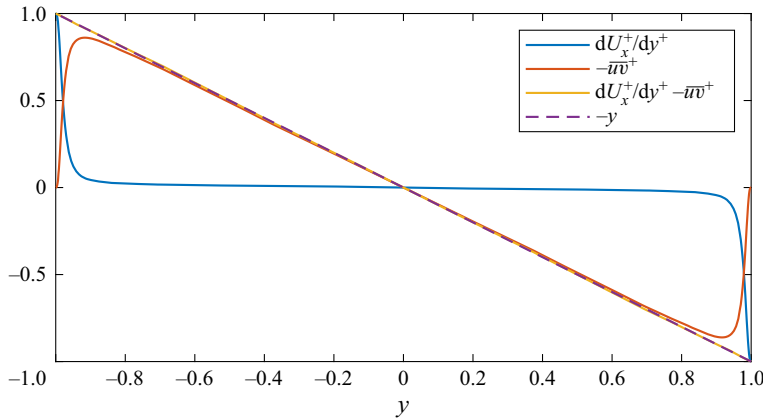
Figure 1. Momentum budget plot for the DNS of the channel flow.
