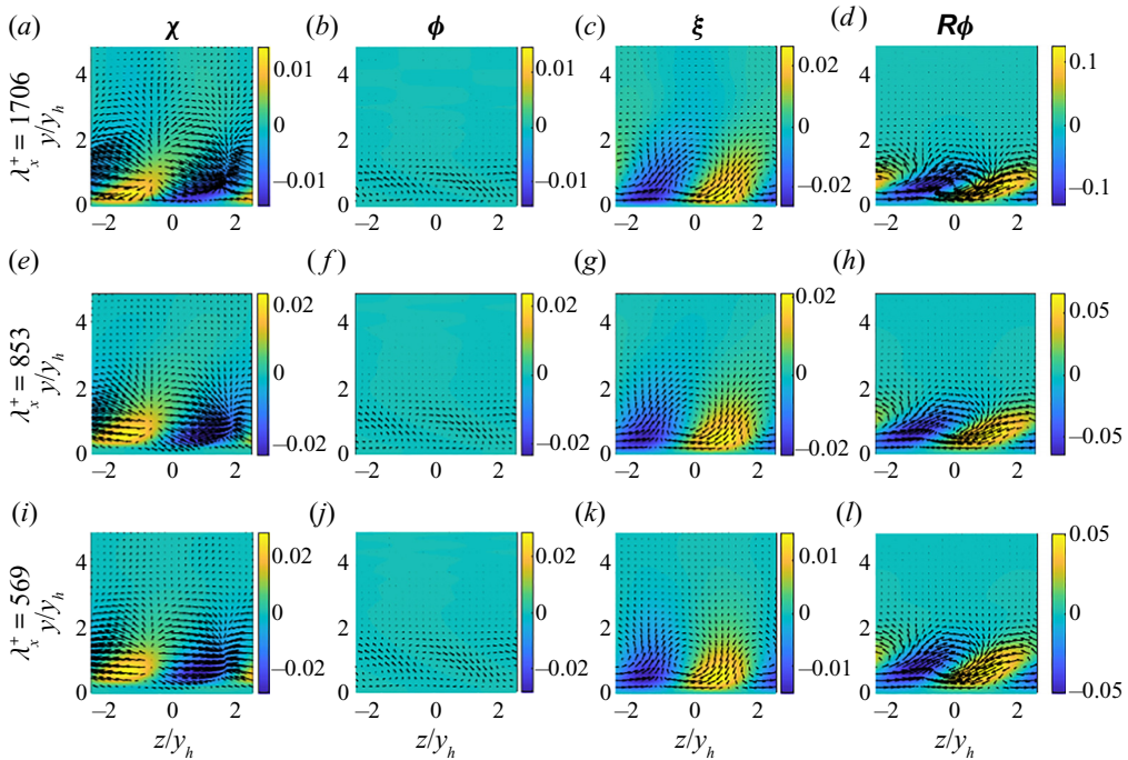
Figure 9. Reconstruction of wall-shear-associated forcing modes \chi (a,e,i) and \phi (b,f,j), and the corresponding velocity fields ((c,g,k) and (d,h,l), respectively) in the y - z plane at three wavenumbers (from top to bottom). Colour plots indicate the x -component, while vectors show y - and z -components. The domain is rescaled using y_h for each wavenumber.
