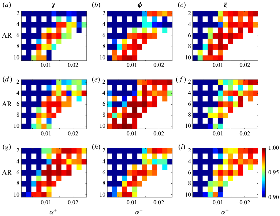
Figure 18. Self-similarity maps \gamma_\chi (a,d,g), \gamma_\phi (b,e,h) and \gamma_\xi (c,f,i), for different ARs and \alpha^+ values, obtained at sub-dominant frequencies. Panels (a-c), (d-f) and (g-i) correspond to the x -, y - and z -components, respectively.
