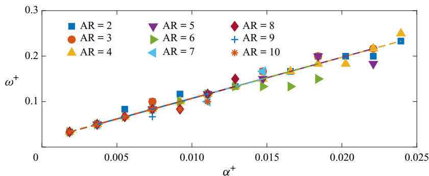
Figure 10. Peak-energy-containing frequencies for different wavenumber pairs with fixed AR. Different markers indicate different AR values. The coloured dashed lines correspond to the best-fit lines for different ARs, using the same colour code.
