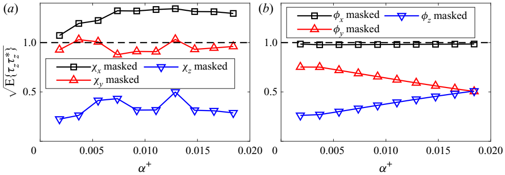
Figure 7. Square root of PSD of \tau_z obtained using partially masked \chi (a) and \phi (b) at different wavenumbers, with AR = 6. Unmasked PSDs are all unity, shown by the dashed lines.
