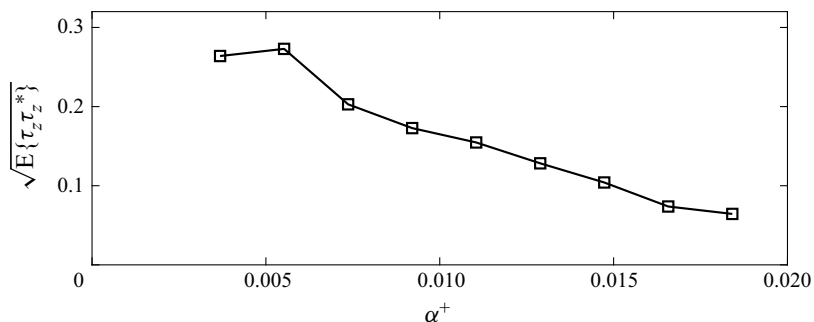
Figure 5. Amplitude spectral density of spanwise wall shear \tau_z at \omega_{max} for different Fourier-mode pairs with AR = 6.
