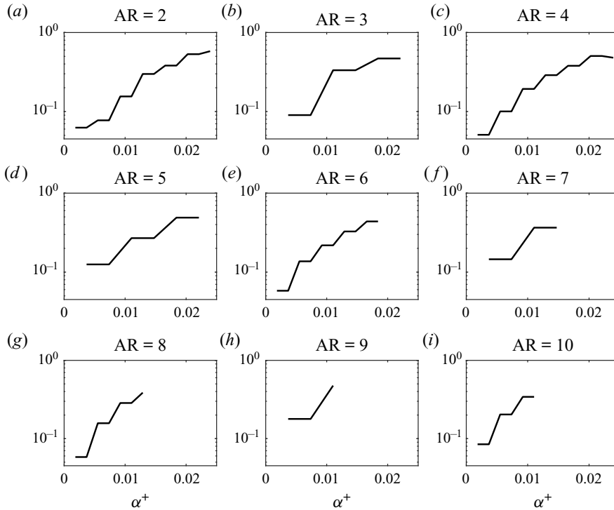
Figure 16. Ratio of the amplitude of \tau_z calculated at sub-dominant frequencies to that calculated at \omega_{max} at different wavenumbers.
