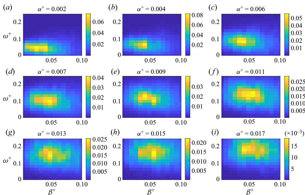
Figure 2. PSD map of \tau_z for different \alpha^+ values.
