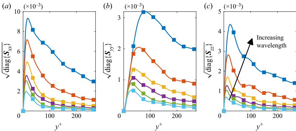
Figure 4. PSD of the response \hat{q} (solid lines) in comparison to its resolvent-based prediction R\hat{f} (markers) at \omega_{max} for different Fourier-mode pairs with AR = 6 . Wavelengths plotted are \lambda_x^+ = 487, 569, 683, 853, 1137 and 1706 .
