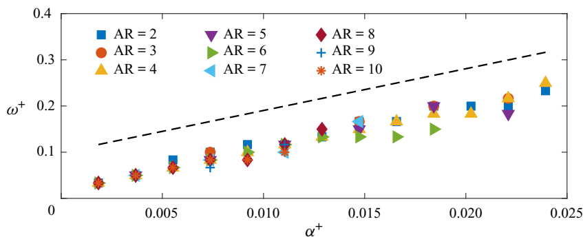
Figure 15. Shifted trend line for \omega^+ corresponding to sub-dominant wall-shear structures.
