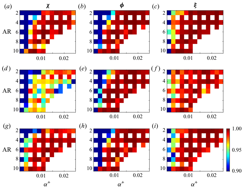
Figure 12. Self-similarity maps \gamma_\chi (a,d,g), \gamma_\phi (b,e,h) and \gamma_\xi (c,f,i), for different ARs and \alpha^+ values. Panels (a–c), (d–f) and (g–i) correspond to the x-, y- and z-components, respectively.
