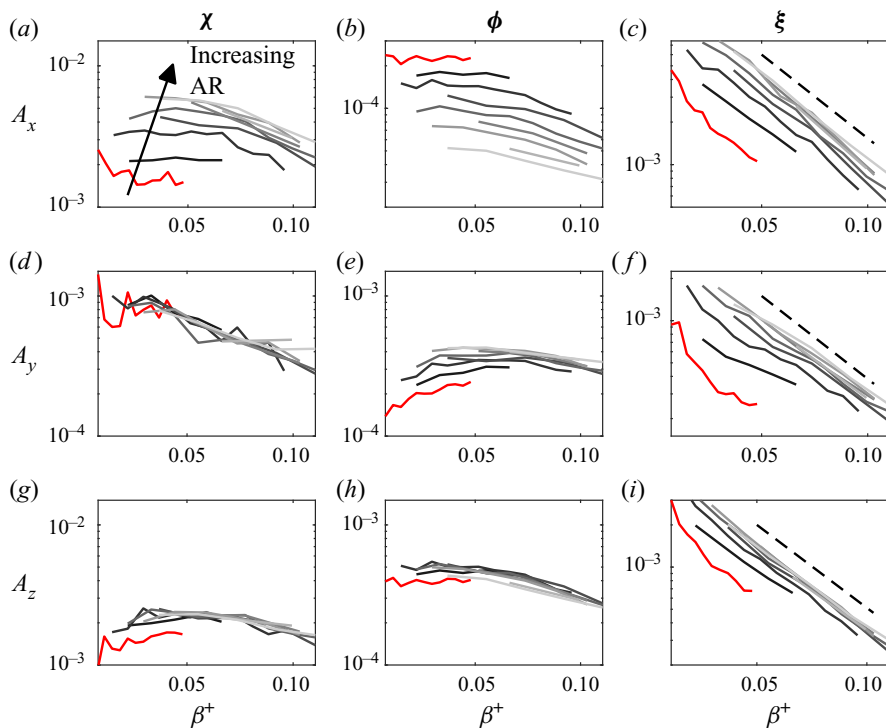
Figure 14. Mode amplitudes for \chi (a,d,g), \phi (b,e,h) and \xi (c,f,i) at different wavenumber pairs. Panels (a–c), (d–f) and (g–i) correspond to the x-, y- and z-components, respectively. ARs range from 2 to 10; AR = 2 is shown in red, and the rest with greyscale. Dashed lines indicate the 1/(\beta^+)^2 trends.
