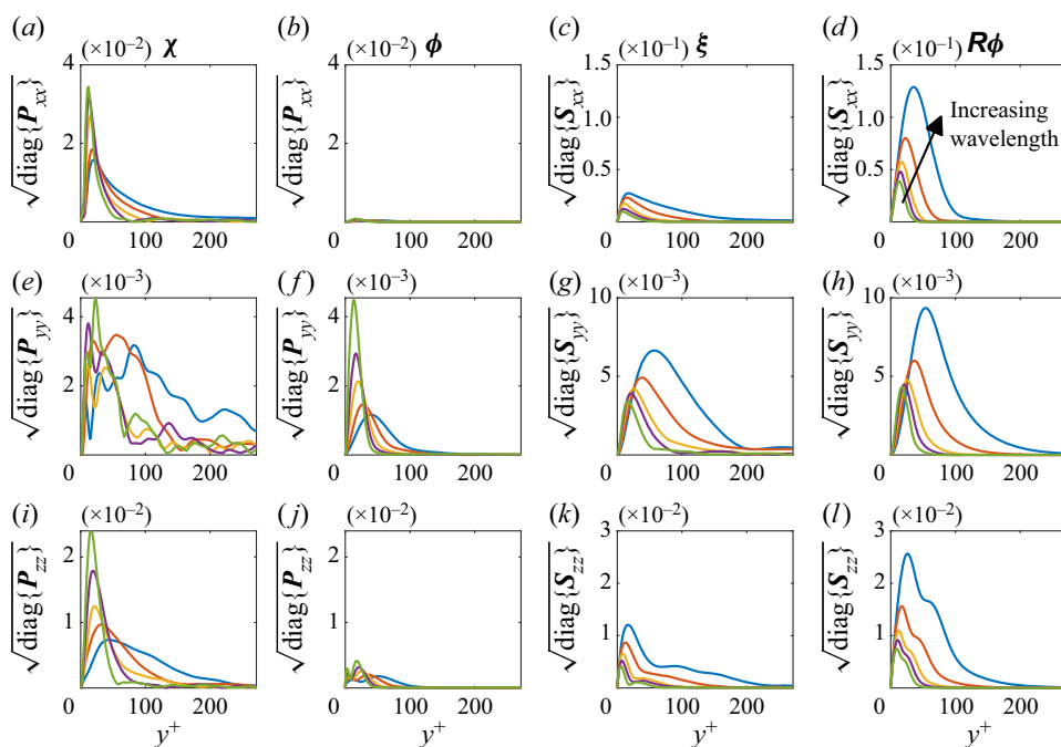
Figure 6. Comparison of the wall-shear-associated forcing modes obtained by RESPOD (a,e,i) and RBE (b,f,j), and the corresponding velocity fields ((c,g,k) and (d,h,l), respectively), at \lambda_x^+ = 341, 487, 682, 1137 and 1706, with \lambda_x^+/\lambda_z^+ = 6 .
