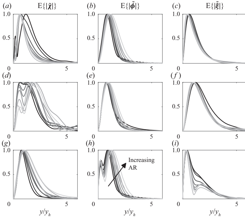
Figure 13. Mean self-similar modes for \chi (a,d,g), \phi (b,e,h) and \xi (c,f,i). Panels (a–c), (d–f) and (g–i) correspond to the x -, y - and z -components, respectively.
