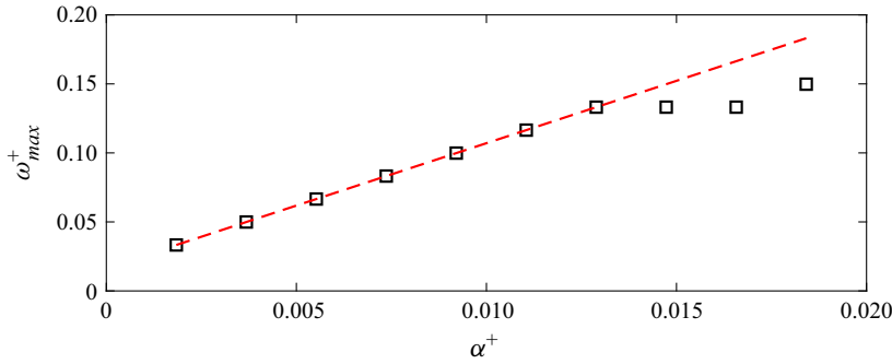
Figure 3. Maximum-energy-containing frequency, \omega_{max} , of spanwise wall shear \tau_z for different Fourier-mode pairs with AR = 6 . The red dashed line indicates the best fit minimising L_1 -norm error.
