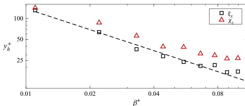
Figure 8. Mode centre y_h^+ obtained using \xi_x (square) and \chi_z (triangle) at different wavenumbers, with AR = 6. The dashed line shows the 1/\beta^+ trend.
