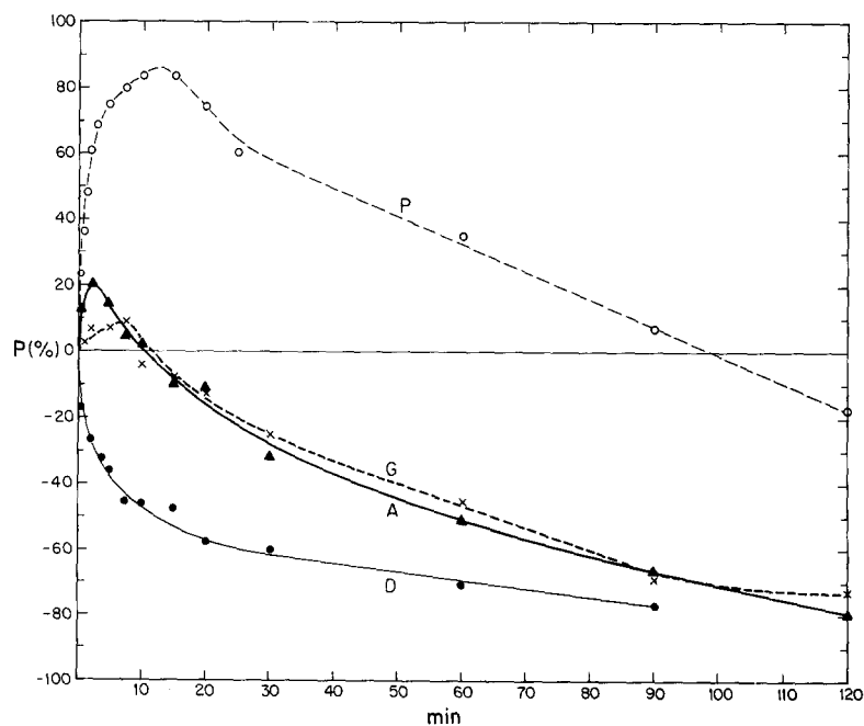
Fig. 2. Percentage change in absorbance P (%) as a function of grinding time for bands A (▲—▲—▲), D (●—●—●), G (×—×—×) and P (○—○—○).
