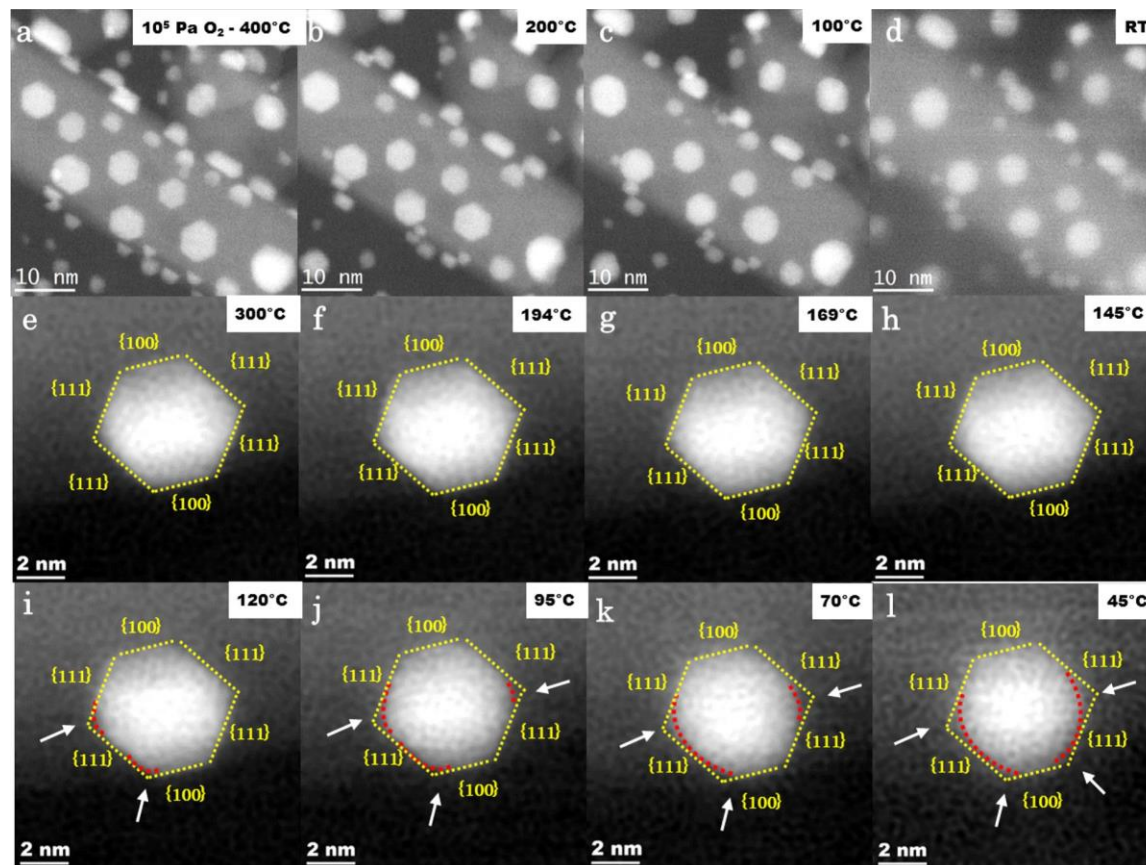
Figure 2. In situ HAADF-STEM observations of Au nanoparticles on r-TiO 2 (110) surfaces under O 2 at atmospheric pressure. (a-d) Temperature series of low magnification HAADF-STEM images showing that rounding of Au nanoparticles at low temperature. (e-l) Temperature series of high magnification HAADF-STEM images over the temperature window where the octahedron-to-round morphology transition is observed. This shape transition is due to the growth of (110) facets on which O 2 molecules preferentially react. Extracted with permission from ref. [3].
