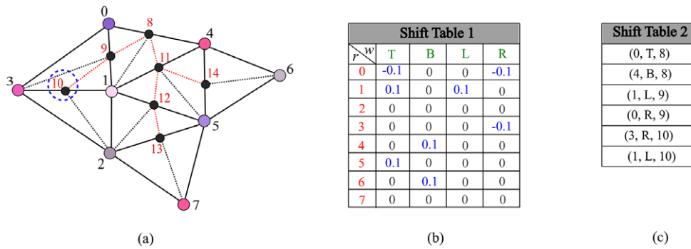
Figure 10. Iteration 3: (a) Considering the triplet (10, 3, 1) with corridor vertex 8 from G_C , (b) Shift Table 1 at the end of iteration 3, and (c) Shift Table 2 at the end of iteration 3.
