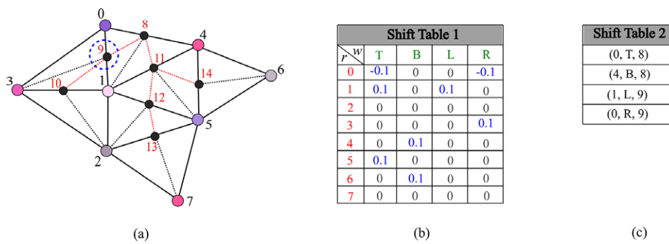
Figure 9. Iteration 2: (a) Considering the triplet (9, 0, 1) with corridor vertex 9 from G_C , (b) Shift Table 1 at the end of iteration 2, and (c) Shift Table 2 at the end of iteration 2.
