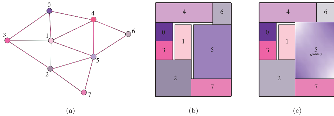
Figure 18. (a) The input graph. (b) The spanning circulation (like mentioned in previous algorithm the entry corridor, here 0 – 1, is not explicitly shown since it is known to be a door). (c) The corridor placement if the room 5 alone is made public .
