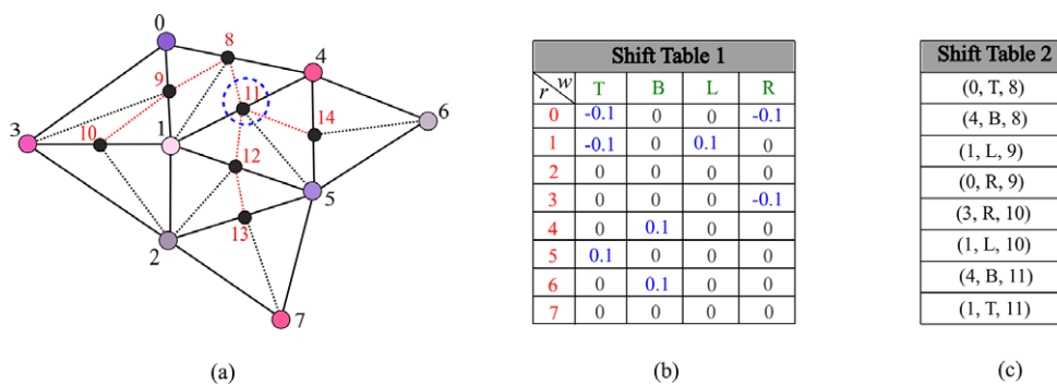
Figure 11. Iteration 4: (a) Considering the triplet (11, 1, 4) with corridor vertex 11 from G_C , (b) Shift Table 1 at the end of iteration 4, and (c) Shift Table 2 at the end of iteration 4.
