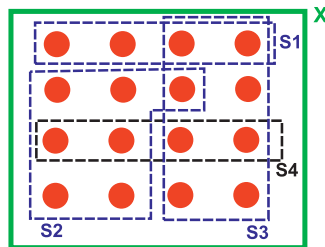
Figure 13. An instance of minimum set cover to illustrate Algorithm 4.
