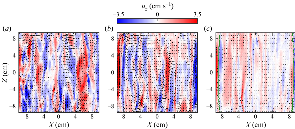
Figure 4. Instantaneous flow fields for \gamma = 3.50 , (a) \Omega = 20 r.p.m., (b) 27 r.p.m. and (c) 40 r.p.m.. All three figures share the same colour bar. The dark green solid lines in (c) indicate the edges of the hot and cold coherent structures near the sidewall.
