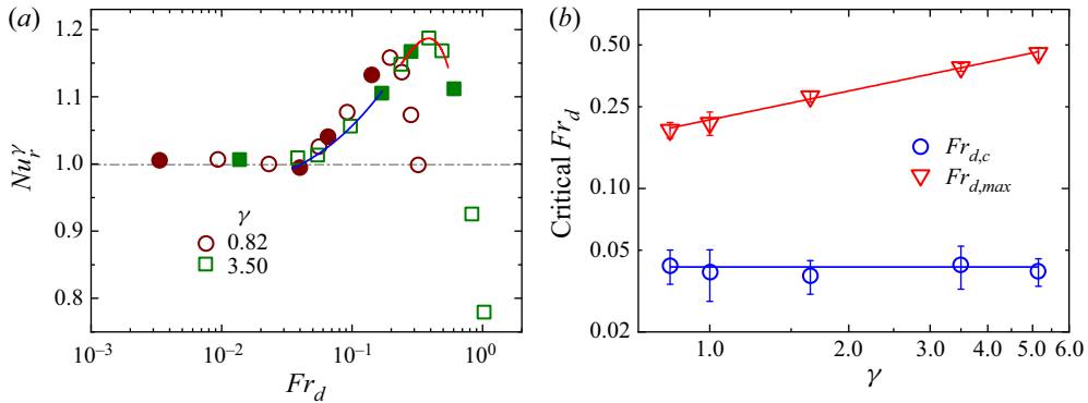
Figure 2. (a) The reduced Nusselt number Nu_r^\gamma as a function of Fr_d for \gamma = 0.82 and 3.50 . The onset ( Fr_{d,c} ) and optimal ( Fr_{d,max} ) Froude numbers are defined, respectively, as the intersection of a logarithmic fitting (blue solid line) and the baseline Nu_r^\gamma = 1.0 and the peak of a parabolic fitting (red solid line). To relate the heat transport enhancement to the changes of flow fields in figure 3 conveniently, the cases that PIV measurements were also performed are indicated here by solid symbols. (b) The onset and optimal Froude numbers as a function of \gamma . The blue solid line indicates the mean value of the onset Froude number Fr_{d,c} = 0.04 . The red solid line is a power-law fitting, Fr_{d,max} = 0.22\gamma^{0.47\pm 0.02} . The error bars are the fitting errors.
