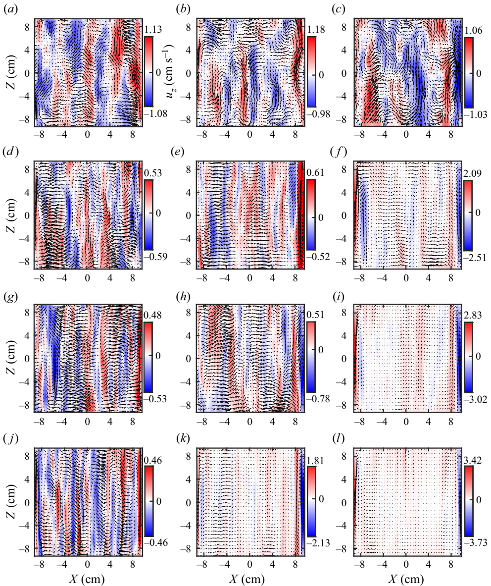
Figure 3. Time-averaged velocity fields for \gamma = 0.00 (a,d,g,j), 0.82 (b,e,h,k) and 3.50 (c,f,i,l), and for each \gamma , \Omega = 6 r.p.m., 20 r.p.m., 27 r.p.m. and 40 r.p.m. (from (a–c) to (j–l)). The corresponding parameters [1/Ro, Fr_d] for each map are (a) [2.28, 0]; (b) [2.28, 0.003]; (c) [2.28, 0.01]; (d) [7.62, 0]; (e) [7.59, 0.04]; (f) [7.57, 0.15]; (g) [10.23, 0]; (h) [10.21, 0.07]; (i) [10.17, 0.28]; (j) [15.19, 0]; (k) [15.25, 0.14]; (l) [15.11, 0.61]. The colour bars are coded by the vertical velocity u_z in unit of \text{cm s}^{-1} with the maximum and minimum values indicated in the respective maps.
