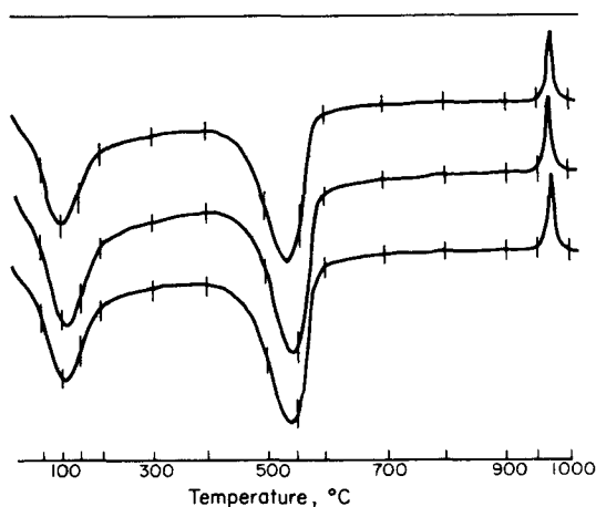
Fig. 2. DTA curves of kaolinite. All curves were made from 15 mg of pelleted samples under the same instrument conditions (300 u.v.; chart speed 0.2 in./min; heating rate 20°C/min; preheat 25 sec).
