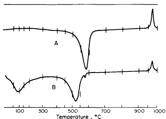
Fig. 4. DTA curves of a mixture of quartz (50 per cent) and kaolinite (50 per cent) showing the difference of reaction temperatures, sensitivity and resolution of the reactions between a large sample (200 mg) packed in a nickel block holder (curve A) and a pelleted sample of semi-micro quantity (15 mg) (curve B). Instrument conditions were the same as in Fig. 2 except curve A, 1200 u.v.
