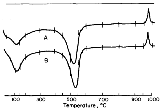
Fig. 3. DTA curves of a mixture of quartz (25 per cent by wt.) and kaolinite (75 per cent by wt.) showing the difference of low temperature endothermic peaks between a sample started with a warm furnace (curve A) and a sample started with a furnace of room temperature (curve B). Other conditions were the same as in Fig. 2.
