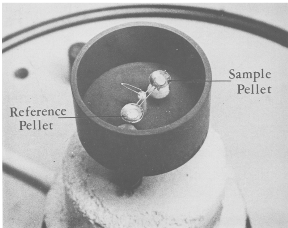
Fig. 1. Pelleted sample and reference material on the platinum dishes in a micro sample holder. Holder diameter 4 cm.
