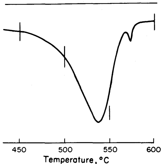
Fig. 5. DTA curve of a mixture of quartz (50 per cent) and kaolinite (50 per cent) packed in a nickel block holder. Sample wt. 200 mg; 1200 u.v.; chart speed 0.1 in./min; heating rate 5°C/min. Compare with Fig. 4.
