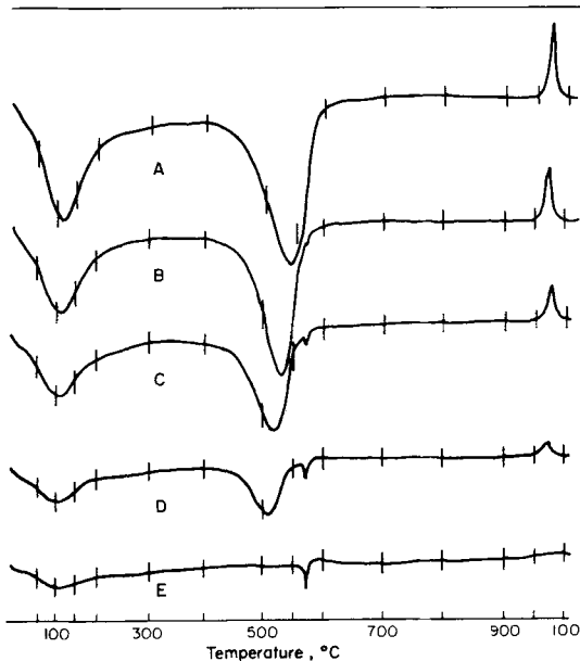
Fig. 6. DTA curves: A, kaolinite 100 per cent; B, kaolinite 75 per cent; quartz, 25 per cent; C, kaolinite 50 per cent; quartz, 50 per cent; D, kaolinite 25 per cent; quartz, 75 per cent; E, quartz, 100 per cent. Sample weight and instrument conditions were the same as in Fig. 2.
