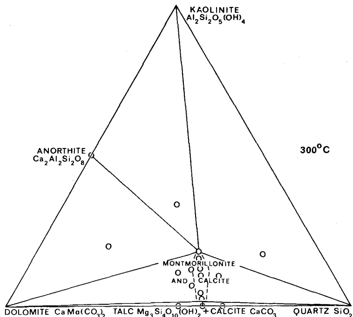
Fig. 1. Dolomite, quartz and kaolinite (equations 1, 2 and 3) react in a hydrous environment at 300°C to form products illustrated in the ternary diagrams. The area within the dotted line represents montmorillonite and calcite. Each circle represents a single bomb reaction.
