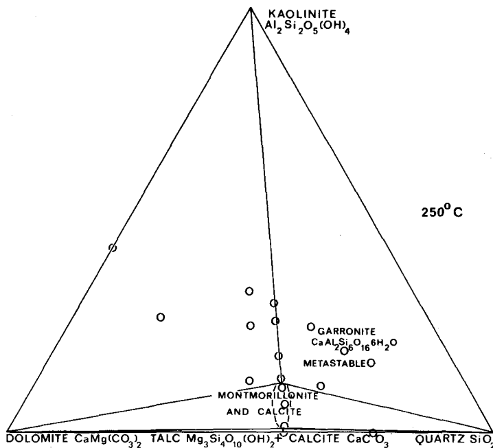
Fig. 2. Dolomite, quartz and kaolinite (equations 1, 2 and 7) react in a hydrous environment at 250°C to form products illustrated in the ternary diagram. The area within the dotted line represents montmorillonite and calcite. Each circle represents a single bomb reaction.
