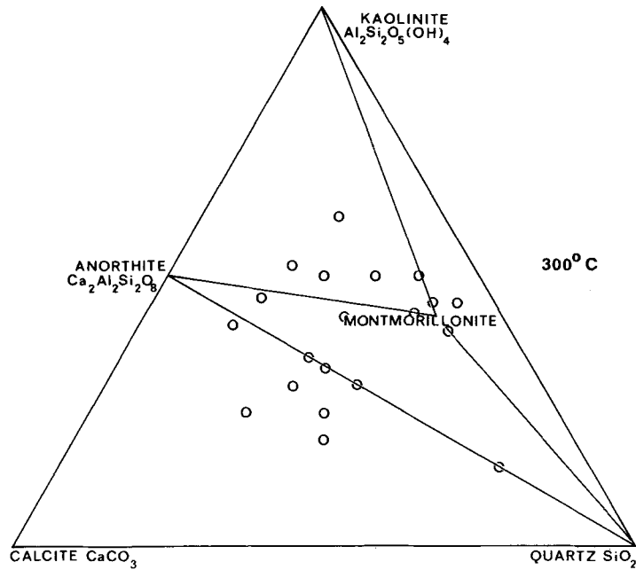
Fig. 3. Calcite, quartz and kaolinite (equations 4 and 5) react in a hydrous environment at 300^\circ\text{C} to form products illustrated in the ternary diagram. Each circle represents a single bomb reaction.
