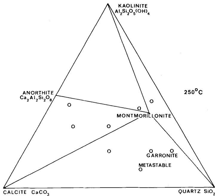
Fig. 4. Calcite, quartz and kaolinite (equations 4-6) react in a hydrous environment at 250^\circ\text{C} to form products illustrated in the ternary diagram. Each circle represents a single bomb reaction.
