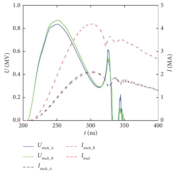
FIGURE 11: Calculated A-level and B-level stack voltage, A-level and B-level stack current, and total current.
