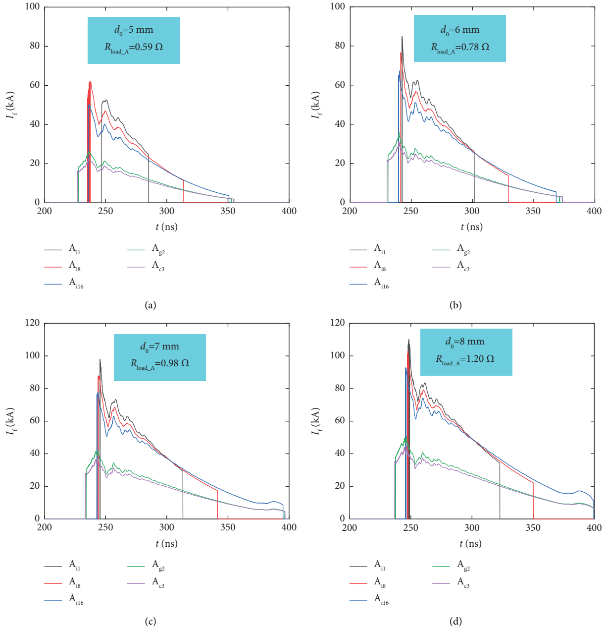
FIGURE 10: Time history of the electron flow currents in each segment of A-level MITL (CRT load). (a) d_0 = 5 mm and R_{load\_A} = 0.59 \Omega . (b) d_0 = 6 mm and R_{load\_A} = 0.78 \Omega . (c) d_0 = 7 mm and R_{load\_A} = 0.98 \Omega . (d) d_0 = 8 mm and R_{load\_A} = 1.20 \Omega .
