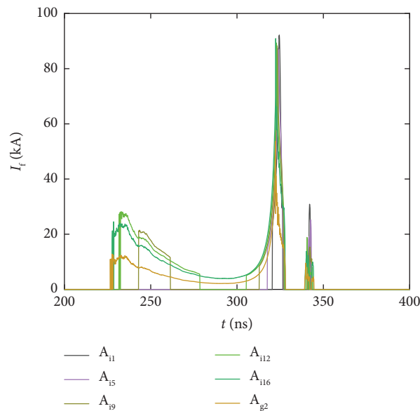
FIGURE 13: Time history of the electron flow currents in each MITL segment of A-level MITL as functions of time (Z-pinch load).
