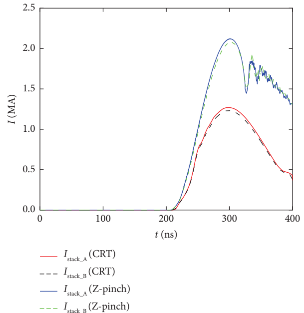
FIGURE 15: Comparison of the stack current for the two loads. The stack current of each level is about 1.3 MA when the accelerator drives the CRT load ( d_0=8 mm, R_{load\_A}=1.20\ \Omega , and R_{load\_B}=1.22\ \Omega ). The stack current of each level is about 2.1 MA when the accelerator drives the Z-pinch load ( l=1.5 cm, r_0=1.2 cm, and mass = 0.3 mg/cm).
