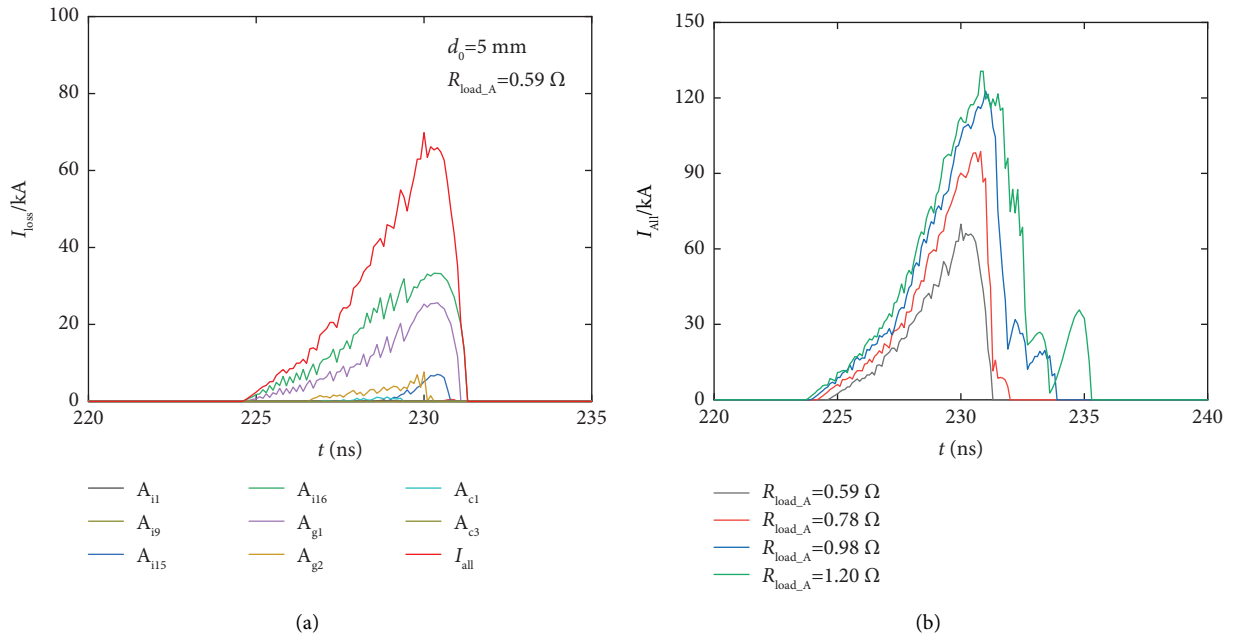
FIGURE 9: (a) Electron current loss in each segment of the A-level MITL when d_0 = 5 mm and R_{load,A} = 0.59 \Omega . (b) Comparison of total loss current when driving different load impedances. The total loss current I_{all} is calculated from the sum of the electron-loss current of the segment A_{i1} \sim A_{c3} .
