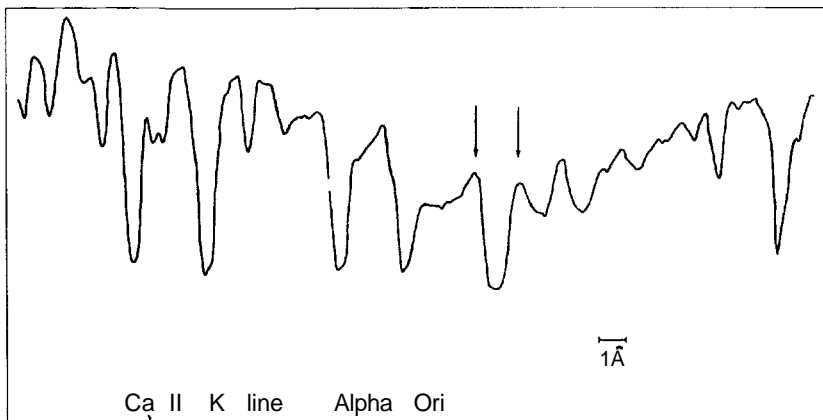
Figure 11-18 Microdensitometer tracing of the Ca II K line in \alpha Ori. The arrows indicate the K_2 peaks.
