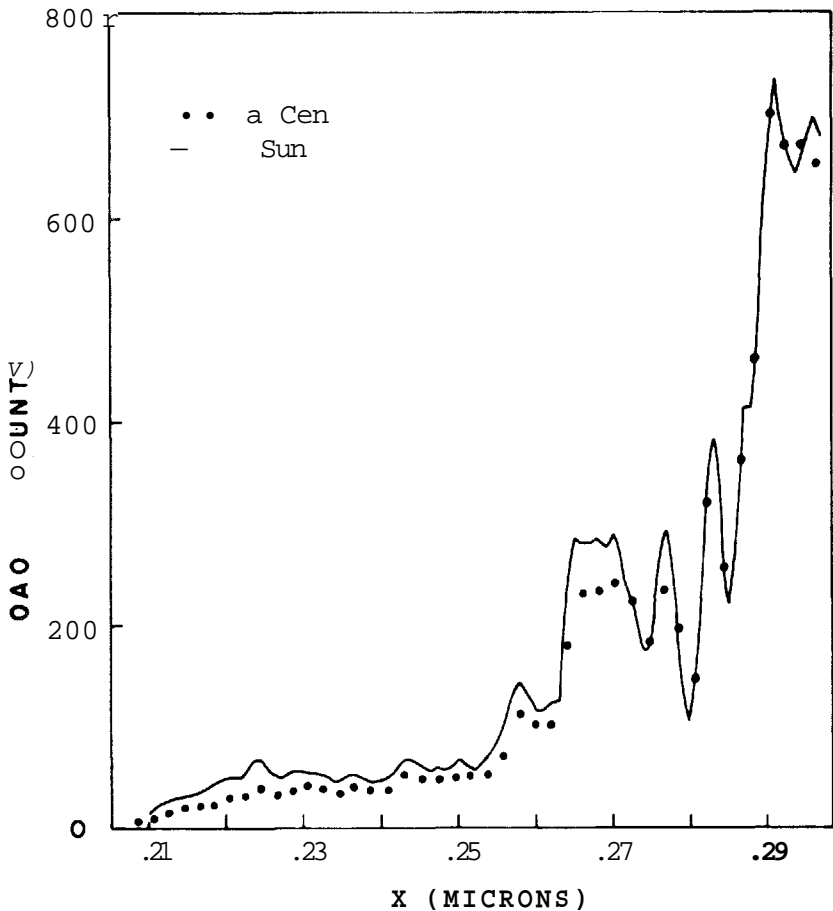
Figure II-2 OAO scan of a Cen compared with the solar spectrum smeared to a resolution of 20 Å and normalized to the scan at 2900 Å
