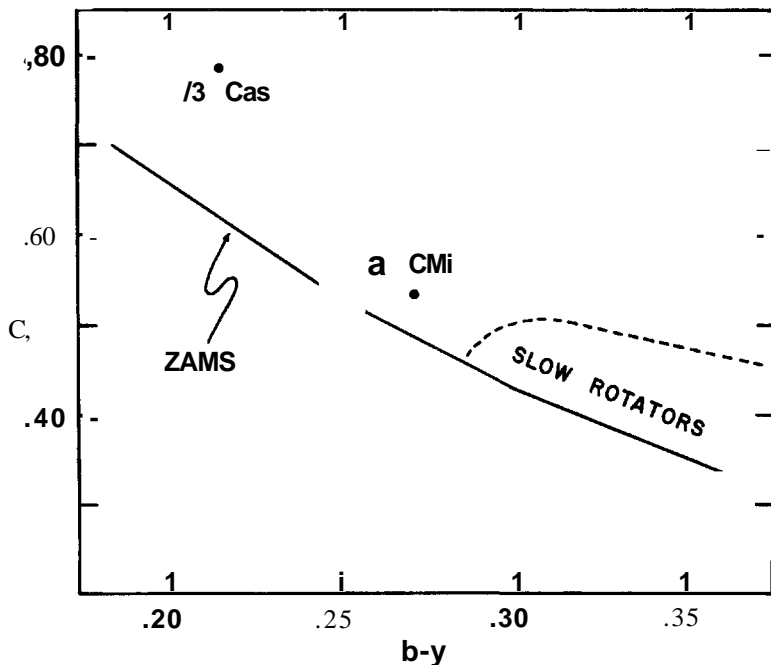
Figure 11-12 c_j -( b-y ) diagram for F stars. The solid line is Stromgren's (1963) Zero Age Main Sequence. The broken line is the boundary between Wilson's (1966) fast and slow rotation regions.
