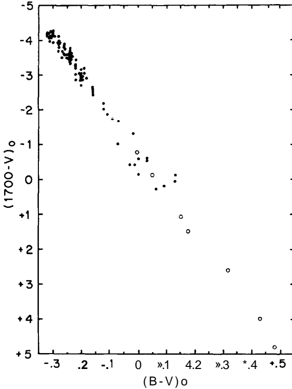
Figure II-7 Stellar X.1700 - V color vs. B-V with 1700 Å wide-band photometry from OAO.
