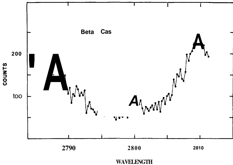
Figure 11-13 Observation of the Mg II lines in j3\text{Cas} on 1971 Oct. 7/8.
