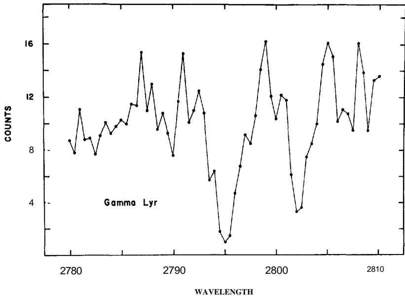
Figure 11-11 Observation of the Mg II lines in \gamma Lyr on 1971 June 6/7.
