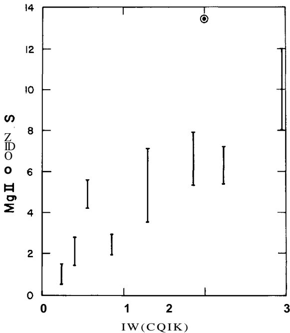
Figure II-6 Mg II A2800 emission (OAO reduced counts) vs. IW, a measure of Call K emission flux at the Earth. The Sun is shown as it would appear if it were a V=0 star measured in the same way.
