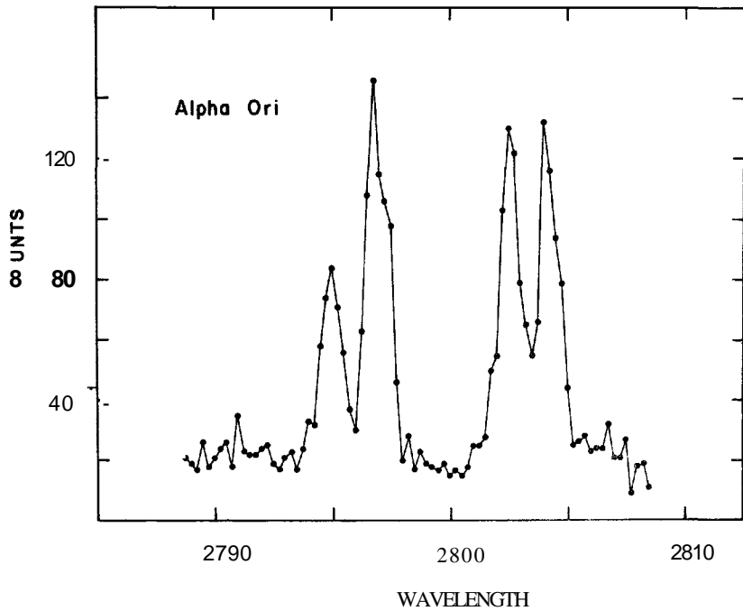
Figure 11-17 Observation of the Mg II lines in \alpha Ori on 1971 Oct. 7/8.
