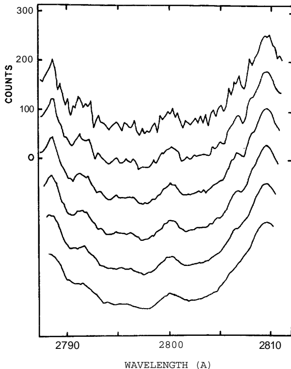
Figure 11-14 The observation of the Mg II lines in j3 Cas smoothed successively over 1, 2, 3,4, 6 and 8 channels.
