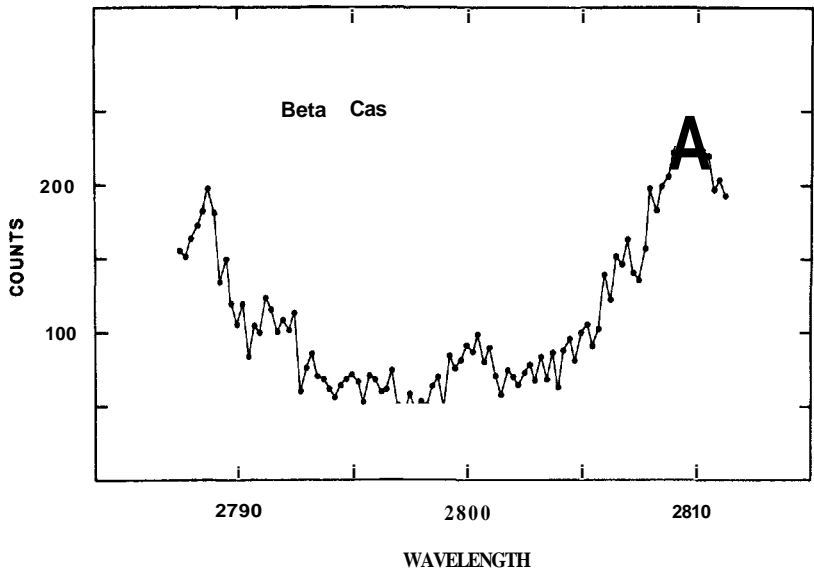
Figure 11-13 Observation of the Mg II lines in \beta Cas on 1971 Oct. 7/8.
