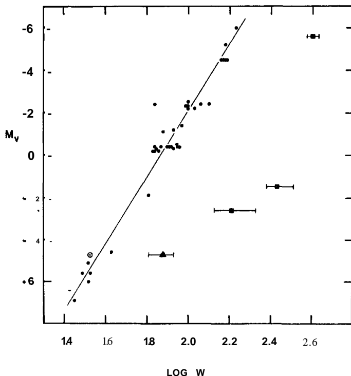
Figure II-19 Plot of M_V versus \text{Log } W , where W is the width of an emission line in \text{km sec}^{-1} . The filled circles are Ca II widths from Wilson and Bappu (1957). The dotted circle is the Ca II width in the Sun (Wilson and Bappu 1957). The squares are Mg II widths in \alpha Ori, \beta Cas and \alpha CMi respectively, in order of decreasing luminosity. The triangle is the solar Mg II width.
