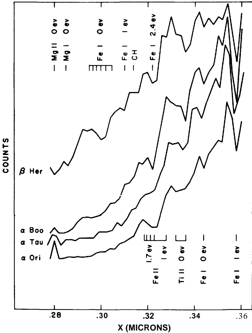
Figure II-3 Changes in ultraviolet spectral features with different spectral type at approximately 25 Å resolution. Ordinate scales are arbitrary. Principal features of the solar spectrum are indicated. \beta Her, G8 III; \alpha Boo, K2 III; \alpha Tau, K5 III; \alpha Ori, M2 lab.
