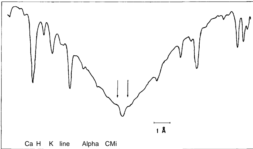
Figure 11-15 Microdensitometer tracing of the Ca II K line in a CMI The arrows indicate the K2 peaks.
