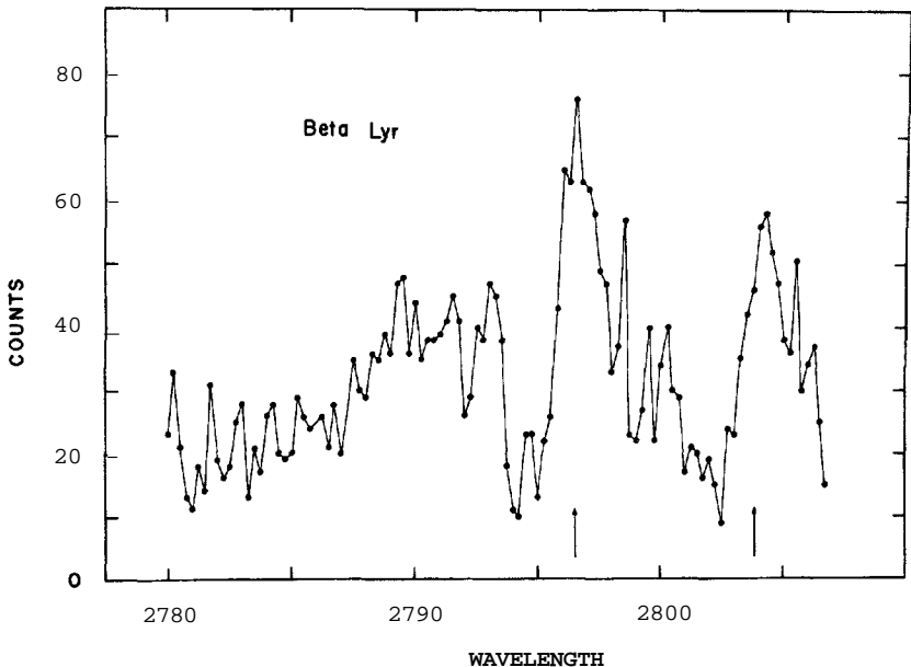
Figure 11-10 Observation of the Mg II lines in \beta Lyr on 1971 June 6/7. The arrows indicate the Mg II line centers at the radial velocity of the B-star component at the time of observation.
