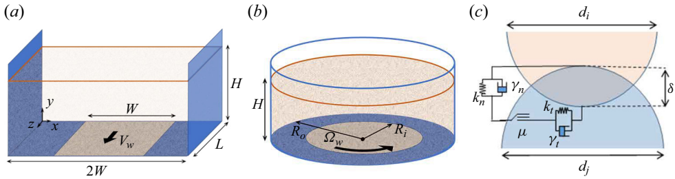
Figure 2. Schematics of the (a) rectangular and (b) cylindrical split-bottom shear cells. The cells are filled to a height H by ‘raining’ the particles from above. In the rectangular device, the middle section of the base of width W translates with a velocity V_w in the z direction, and in the cylindrical device, the central core of radius R_i rotates with angular velocity \Omega_w . (c) Schematic of the interaction model in the discrete element method (DEM). The overlap \delta is exaggerated for clarity.
