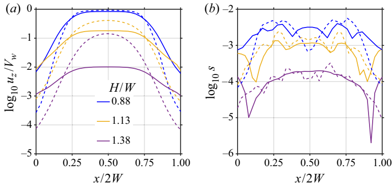
Figure 5. Magnitude of the scaled (a) primary and (b) secondary velocities as a function of x at two heights, y = 0.25H (dashed lines) and y = 0.75H (solid lines) in the rectangular shear cell.
