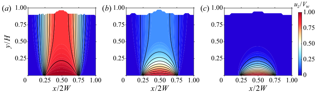
Figure 3. The primary flow obtained from DEM simulations of the rectangular split-bottom shear cell for fill heights H of (a) 0.88W , (b) 1.13W and (c) 1.38W . The colours indicate the scaled velocity u_z/V_w , and the lines are contours of constant velocity in steps of 0.091 .
