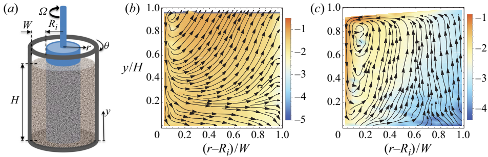
Figure 1. Dilatancy-driven secondary flow in a cylindrical Couette device. The figures are adapted from Krishnaraj & Nott (2016). (a) Schematic of the cylindrical Couette device. (b) Streamlines of the secondary flow at early stages of shear, after a 3.4^\circ rotation of the inner cylinder. (c) The secondary flow at steady state, showing a system-spanning vortex. The colours in panels (b,c) indicate \log_{10} s , where s \equiv (u_r^2 + u_y^2)^{1/2} is the speed of the secondary flow.
