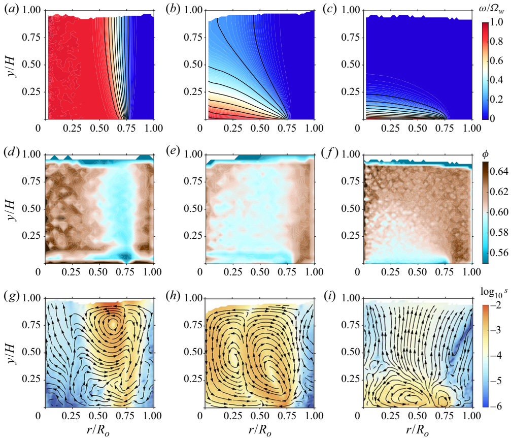
Figure 8. Results of the DEM simulations for the cylindrical shear cell. The figures in each column are for the same fill height H . (a–c) The primary flow for fill heights H of 0.43 R_i , 0.73 R_i and 1.27 R_i . The colours indicate the scaled angular velocity \omega/\Omega_w , and the lines are contours of constant angular velocity in steps of 0.091. (d–f) Colour maps of the particle volume fraction \phi . (g–i) Streamlines of the secondary flow. The colours indicate the speed of the secondary flow s \equiv (u_r^2 + u_z^2)^{1/2}/V_w on a logarithmic scale.
