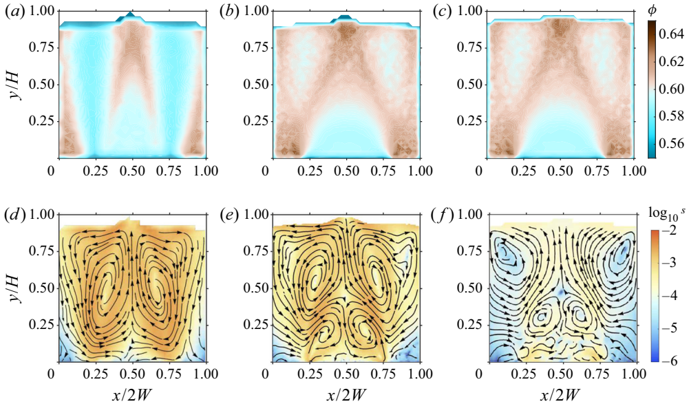
Figure 4. Volume fraction and secondary velocity fields in the rectangular shear cell. (a–c) Colour maps of the particle volume fraction \phi for fill heights H of (a) 0.88W , (b) 1.13W and (c) 1.38W . Regions of very low \phi are coloured white – we have chosen a cutoff of 0.4, but any cutoff less than \approx 0.55 yields the same result. (d–f) Streamlines of the secondary flow for the same fill heights as in figures above. The colours indicate the speed of the secondary flow s \equiv (u_x^2 + u_y^2)^{1/2}/V_w on a logarithmic scale.
