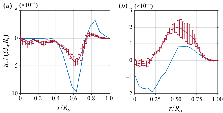
Figure 10. Radial velocity profiles on the free surface in a cylindrical shear cell for fill heights (a) H = 0.43 R_i and (b) H = 0.73 R_i . The red lines with error bars are data from the imaging experiments and the blue lines are the results of DEM simulations.
