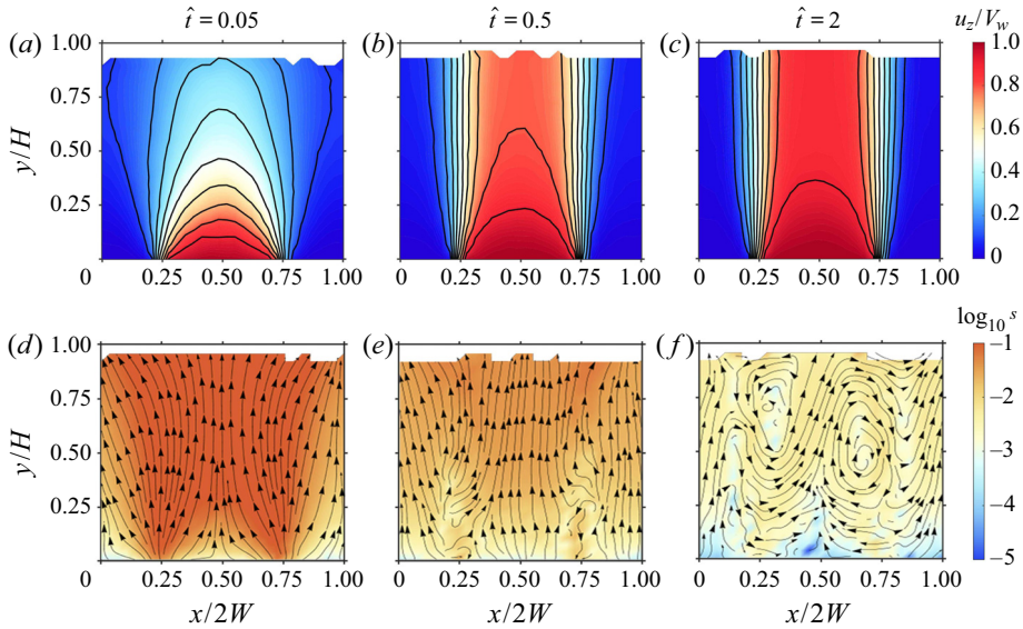
Figure 12. Evolution of the primary and secondary flow fields in time after initiation of shear in a rectangular shear cell with periodic sidewalls for fill height H = 1.38W . Panels (a–c) show colour maps of u_z(x, y) for three dimensionless times \hat{t} \equiv tV_w/W ; the lines are contours of constant u_z in steps of 0.091. Panels (d–f) show streamlines of the secondary flow at the same values of \hat{t} .
