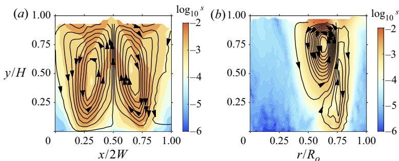
Figure 9. Streamlines of the secondary flow determined as contours of constant stream function \psi , defined in (4.1a,b). (a) Contours of constant \psi in a rectangular shear cell with frictional sidewalls for fill height H = 0.88W . (b) Contours of constant \psi in a cylindrical shear cell for H = 0.43 R_i .
