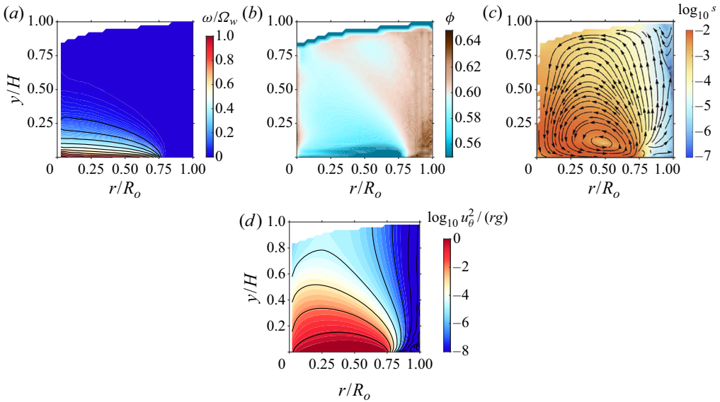
Figure 11. Results of the simulation for H = 1.27R_i at a base rotation speed corresponding to Sa = 8.2 \times 10^{-3} . Colour maps of (a) the primary velocity, (b) particle volume fraction and (c) streamlines of the secondary flow. Panel (d) shows the ratio of the centrifugal and gravitational body forces on a logarithmic scale.
