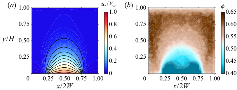
Figure 6. The primary velocity and density fields in the absence of gravity in the rectangular shear cell for fill height H = 0.88W . The figures should be compared with figures 3(a) and 4(a), respectively, that show the two fields for shear in the presence of gravity.
