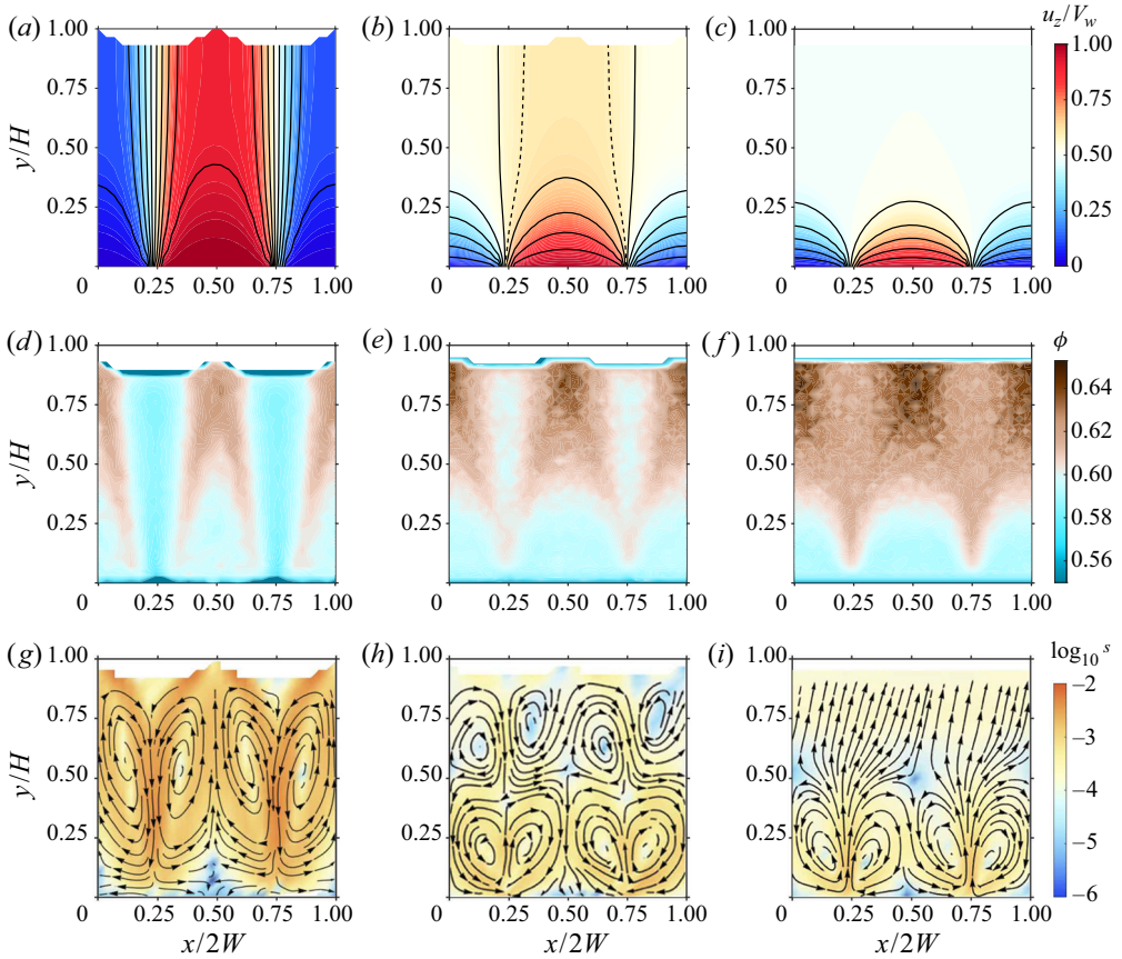
Figure 7. Results of the DEM simulations for a rectangular shear cell with periodic sidewalls. The figures in each column are for the same fill height H . (a–c) The primary flow for fill heights H of 0.88W , 1.13W and 1.38W . The colours indicate the scaled velocity u_z/V_w , and the solid lines are contours of constant velocity in steps of 0.091 . The dashed line in panel (b) is a contour for u_z/V_w = 0.6 . (d–f) Colour maps of the particle volume fraction \phi . (g–i) Streamlines of the secondary flow. The colours indicate the speed of the secondary flow s \equiv (u_x^2 + u_y^2)^{1/2}/V_w on a logarithmic scale.
