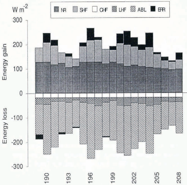
Fig. 4. Energy balance 8–27 July 1993 (Julian days 189–208) at Kronprins Christian Land with net radiation (NR), sensible-heat flux (SHF), latent-heat flux (LHF), conductive-heat flux in the ice (CHF), ablation energy (ABL) and error (ERR). ABL corresponds to stake measurements. ERR appears either on the top or on the bottom depending on whether there is a surplus or deficit of energy. Unit is W m^{-2} .
