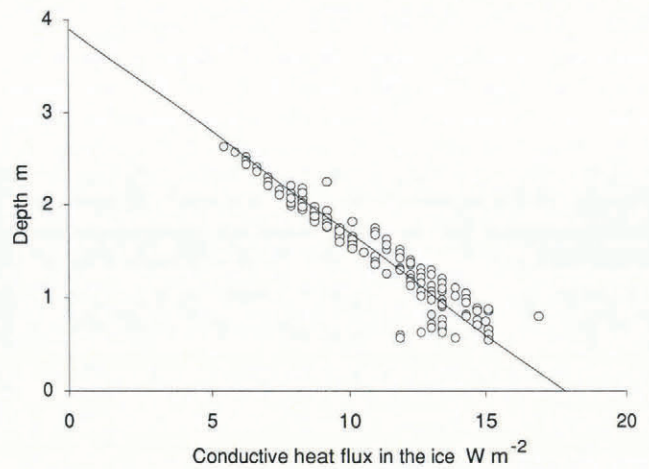
Fig. 3. Calculated conductive heat flux in the ice versus depth below the glacier surface, 8–27 July 1993.
