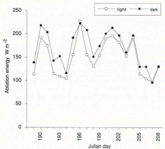
Fig. 2. Ablation energy for “light” and “dark” stakes, 8–27 July 1993 (Julian days 189–208), at Kronprins Christian Land. Unit is \text{W m}^{-2} .
