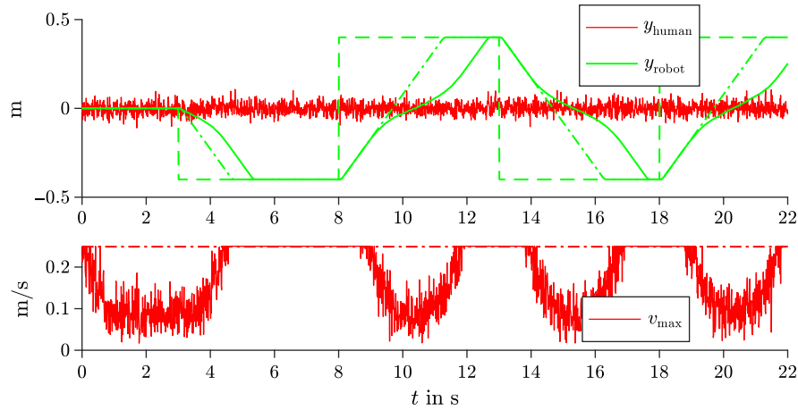
Fig. 5. Hardware Experiment: distance-sensitive v_{\max}(d_{\text{HR}}) with \sigma = \frac{d_{\min}}{3} . Dashed lines are set points, dash-dotted lines result from a constant v_{\max} , and solid lines from v_{\max}(d_{\text{HR}}) as defined in (80). The OTG clearly slows down whenever the distance becomes smaller d_{\min} = 20 cm and uses the user-defined constraint v_{\max} otherwise.
