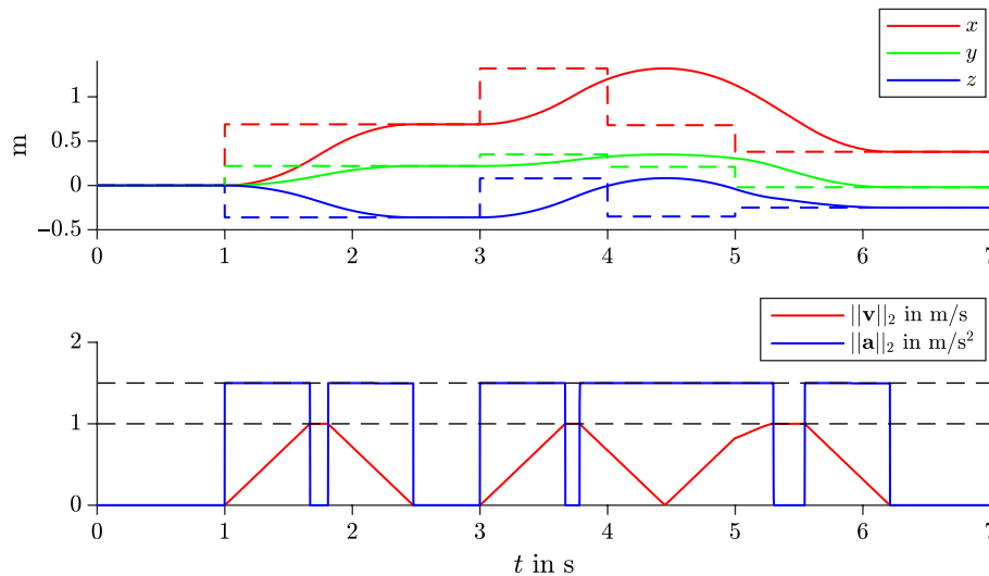
Fig. 6. Trajectory generation for translation with hanging transition. Dashed lines are set points/constraints and solid lines are the actual time-synchronized values. The spikes in acceleration result from the transition phase due to time discretization. The change in set point at t = 5 s causes an adjustment in the direction of the acceleration vector, while its full magnitude a_{\max} = 1.5 \text{ m/s}^2 is still exploited.
