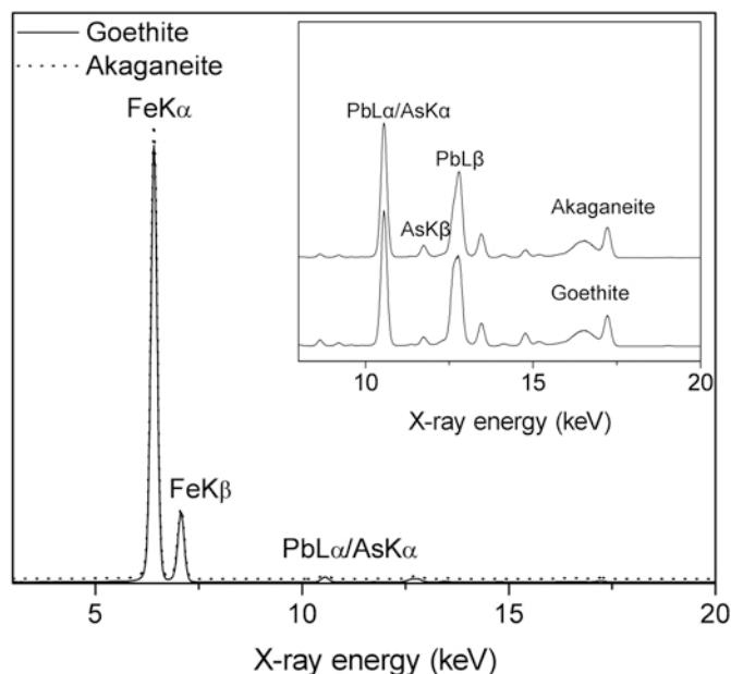
Figure 8. Synchrotron X-ray fluorescence (SXRF) spectra of soil aggregates from the surface precipitates with goethite and akaganeite as the major mineral phases. The inset figure shows the small spectral region of As and Pb fluorescence peaks.
