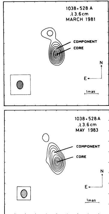
Figure 1. Evolution of the structure of the quasar 1038+528 A. A component is moving out of the core. The core itself appears (nearly) stationary with respect to the quasar 1038+528 B. Contours in both maps correspond to 2, 5, 10, 18, 30, 50, 65, 85, and 95% of the peak of brightness.
