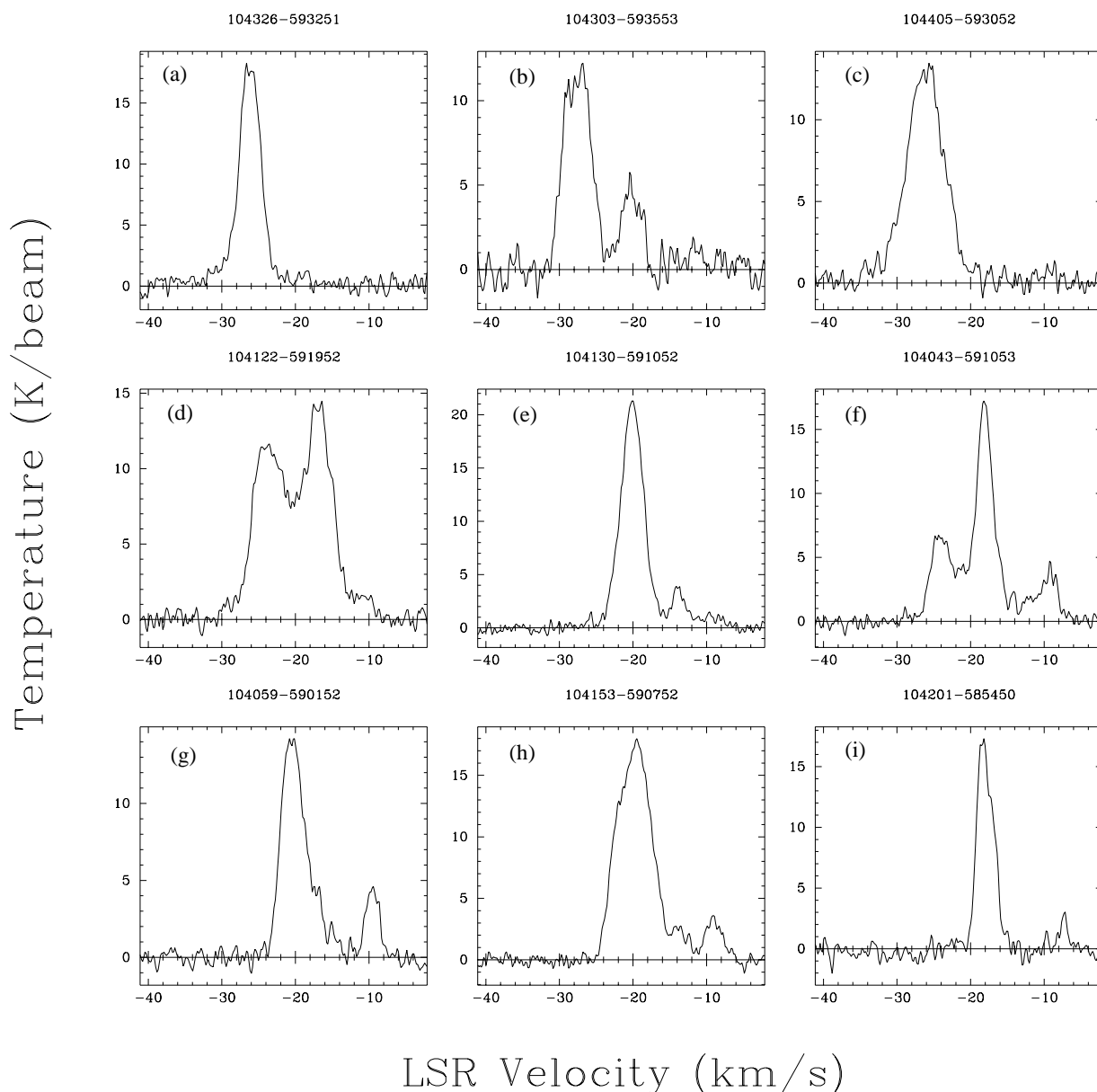
Figure 2 —Typical spectra of the ^{12}\text{CO}(1-0) emission at nine positions throughout the northern and southern cloud. Positions are given in B1950 coordinates.
