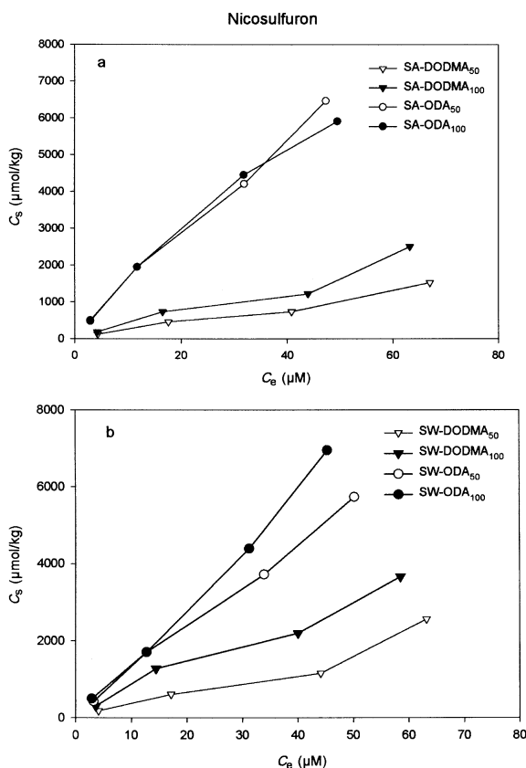
Figure 3. Nicosulfuron sorption isotherms on organoclays: (a) SA-organoclays; (b) SW-organoclays.
