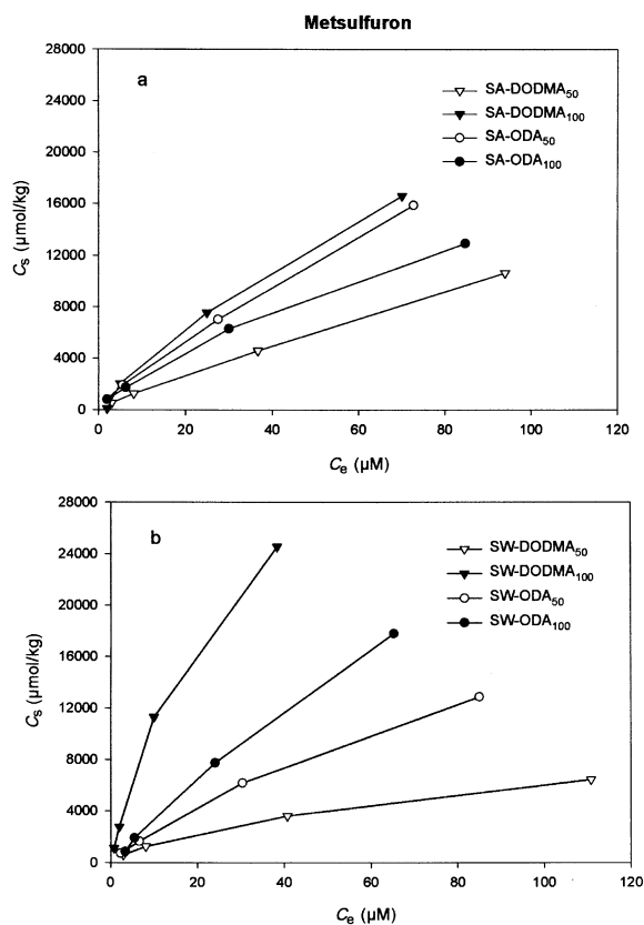
Figure 2. Metsulfuron methyl sorption isotherms on organoclays: (a) SA-organoclays; (b) SW-organoclays.
