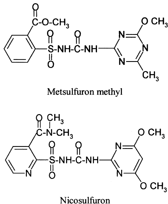
Figure 1. Chemical structures of metsulfuron methyl and nicosulfuron.
