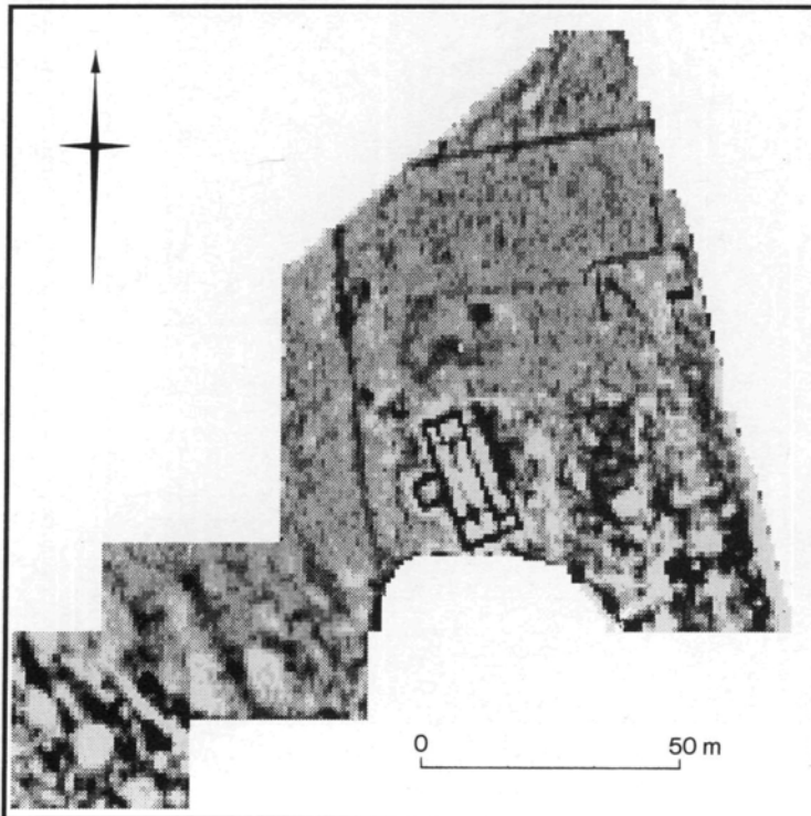
B. Resistivity survey showing the plan of a winged corridor villa at New Farm, South Wanborough. (p. 437) (Photo: RCHME)
