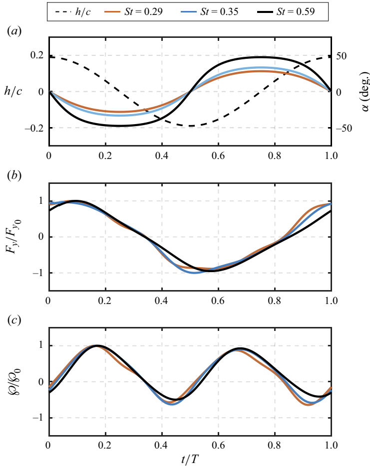
Figure 14. Dimensionless heave cycle h/c (dotted line) and effective angle of attack \alpha (solid lines) for one cycle (a), together with phase-averaged lift forces F_y (b) and power requirements \varphi (c) normalized by maximum values ( F_{y0} and \varphi_0 ) for St = 0.29 (red), St = 0.35 (blue) and St = 0.59 (black).
