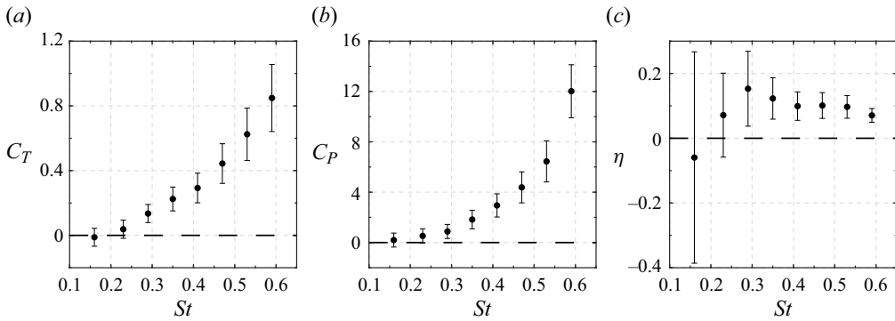
Figure 4. Comparison of time-averaged thrust coefficients and propulsive efficiencies as a function of Strouhal number.
