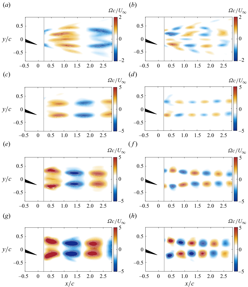
Figure 8. Vorticity fields from opt-DMD modes 1 ( a,c,e,g ) and 2 ( b,d,f,h ) for ( a,b ) St = 0.16 , ( c,d ) St = 0.23 , ( e,f ) St = 0.29 and ( g,h ) St = 0.35 . See also supplementary movie 2 and movie 3 available at https://doi.org/10.1017/jfm.2024.446 .
