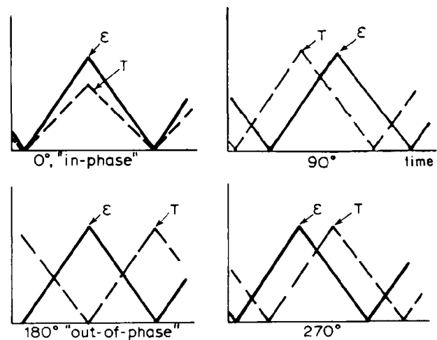
FIG. 9. Timing diagrams illustrating TMF phase relationships. The ordinate represents both applied strain and temperature. Actual applied strain and temperature curves were very similar to those shown.
