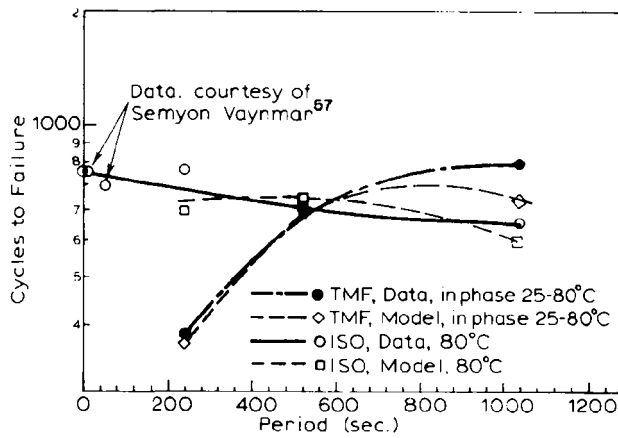
FIG. 5. Effect of period on N_f at 0.6% strain range.
