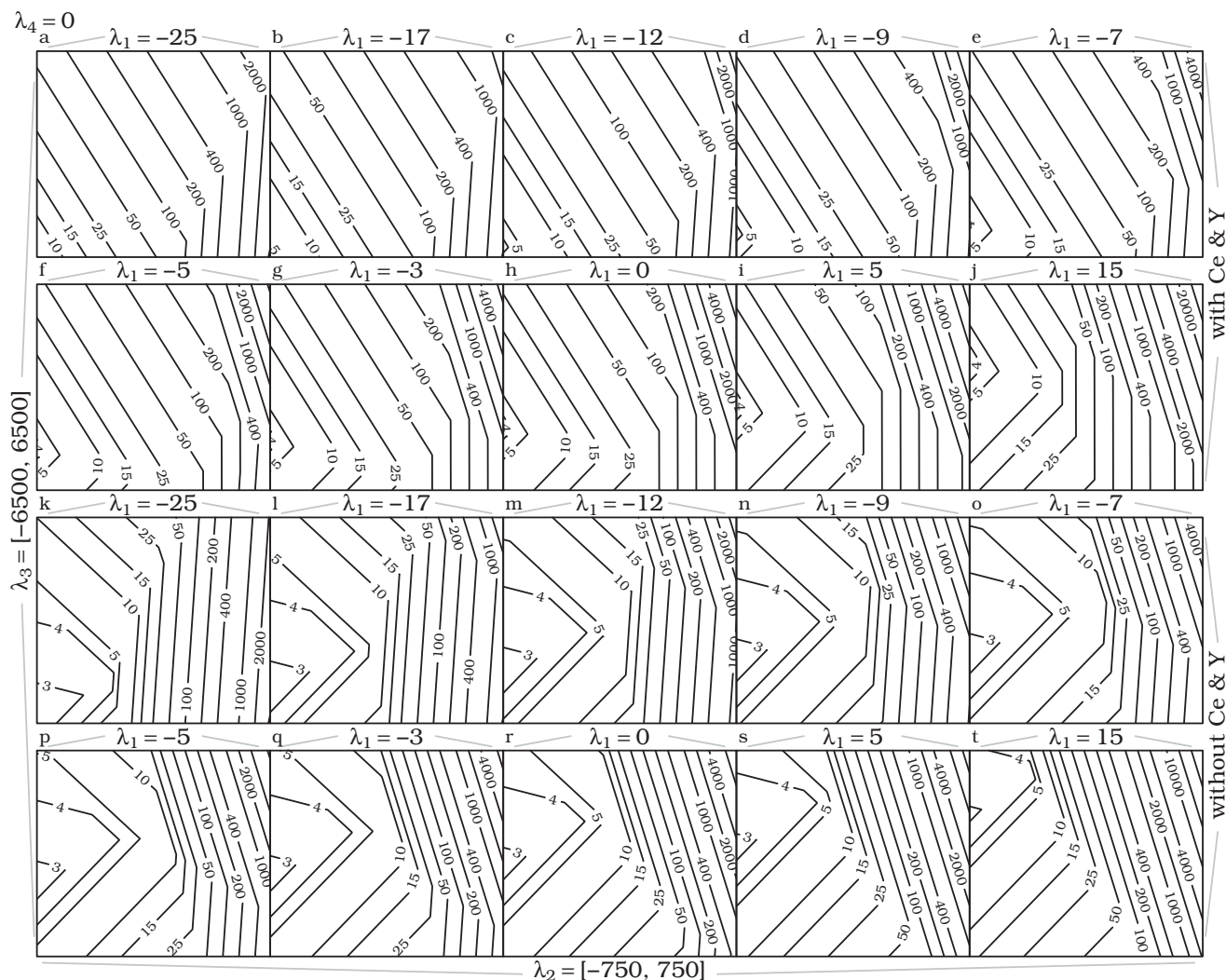
Fig. 6. Contour maps showing the positive Eu anomaly relative to Eu expected from the polynomial required for Eu to be the most abundant REE. Construction of panels is similar to Fig. 3.
