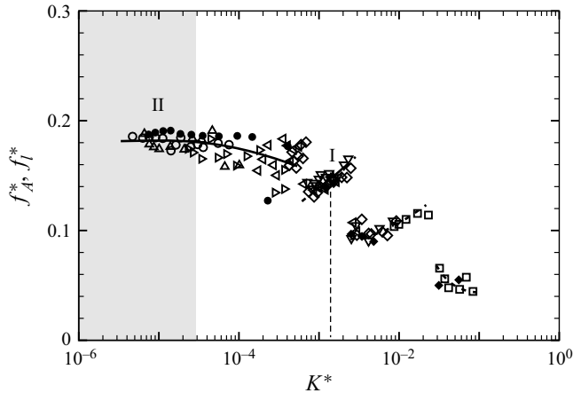
Figure 10. Plot of the variation of the non-dimensional frequencies of flap tip motion ( f_A^* ) and fluctuating lift force ( f_l^* ) vs the effective stiffness ( K^* ). These two frequencies are very well coupled. Solid symbols show lift force frequencies ( f_l^* ), whereas open symbols show flap tip frequencies ( f_A^* ), with different symbols representing the different EI flaps, respectively, as shown in the response plot in figure 6.
