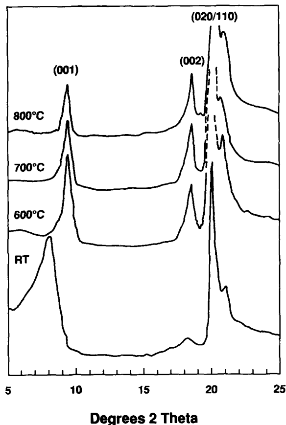
Figure 1. X-ray diffraction pattern of the untreated montmorillonite powder sample at RT and after stepwise heating to 600°, 700°, and 800°C.
