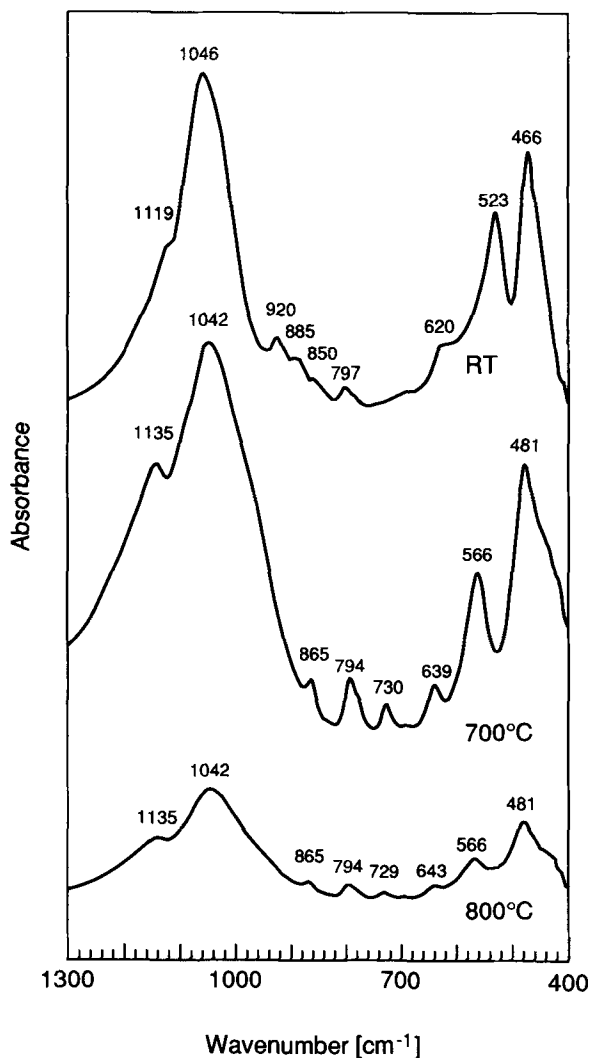
Figure 4. Mid-infrared spectra of the untreated montmorillonite sample at RT and after stepwise heating to 600°, 700°, and 800°C.
