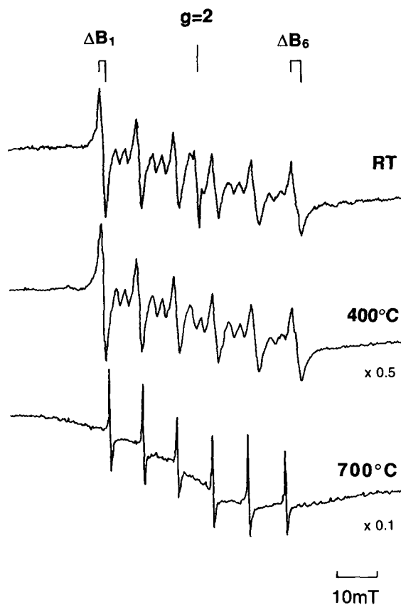
Figure 6. Narrow-range EPR spectra of the untreated montmorillonite sample at RT and after stepwise heating to 400° and 700°C. The spectra of the heat-treated samples are gain reduced by factors of 0.5 and 0.1, respectively.
