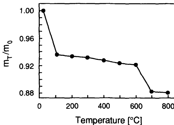
Figure 2. Relative mass loss of the untreated montmorillonite sample during stepwise heating to 800°C for 1 hr at each step.
