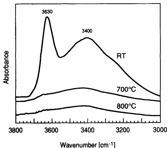
Figure 3. Near-infrared spectra of the untreated montmorillonite sample at RT and after stepwise heating to 600°, 700°, and 800°C.
