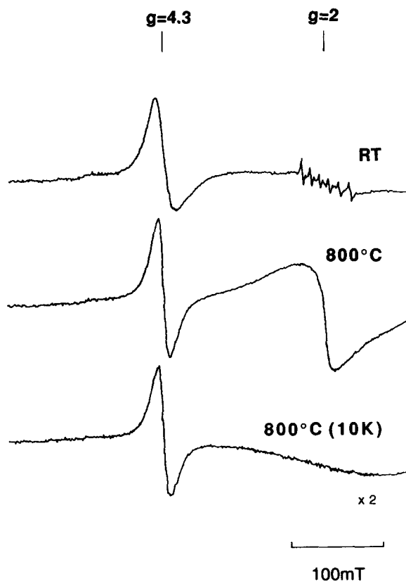
Figure 5. Wide-range EPR spectra of the untreated montmorillonite sample at RT, and after heating to 800°C, measured at RT and 10 K. The low-temperature signal is gain-reduced by a factor of 2.
