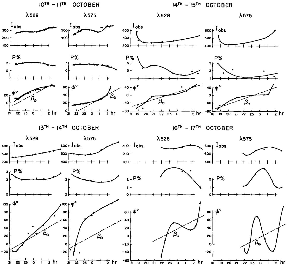
FIGURE 1.—Measured intensity I_{obs} , observed degree P (in percent) and observed angle \phi of polarization in the North ecliptic pole.
