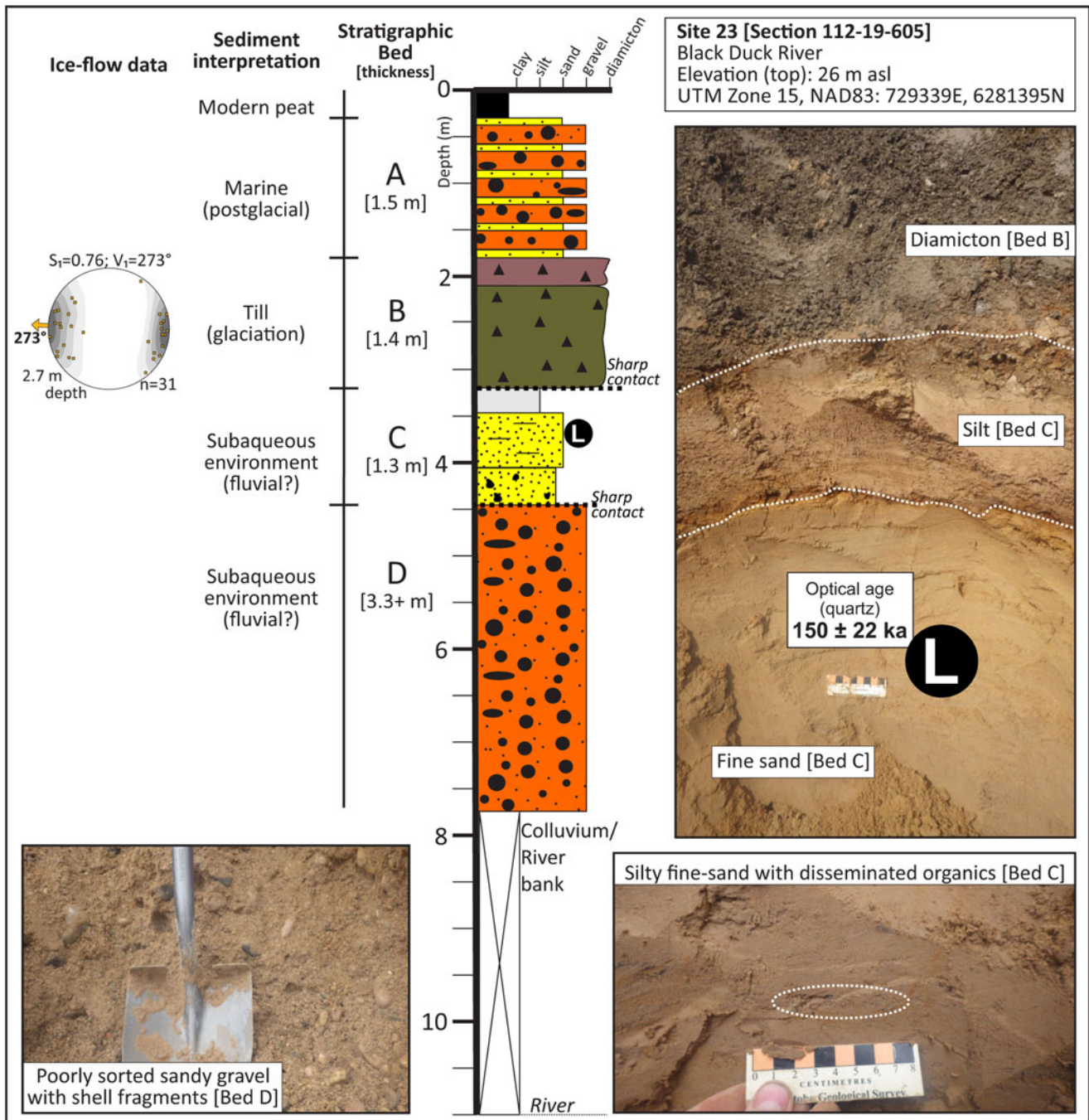
Figure 6. Quaternary stratigraphy and sediment photos of site 23. Till fabric data are plotted on equal area, lower hemisphere projection stereonets, with the principal eigenvalue ( S_1 ) and eigenvector ( V_1 ) values provided. Contours were generated using the Kamb method (Vollmer 1995). The sample location for optical age determination is shown by the black circle with an “L.”
