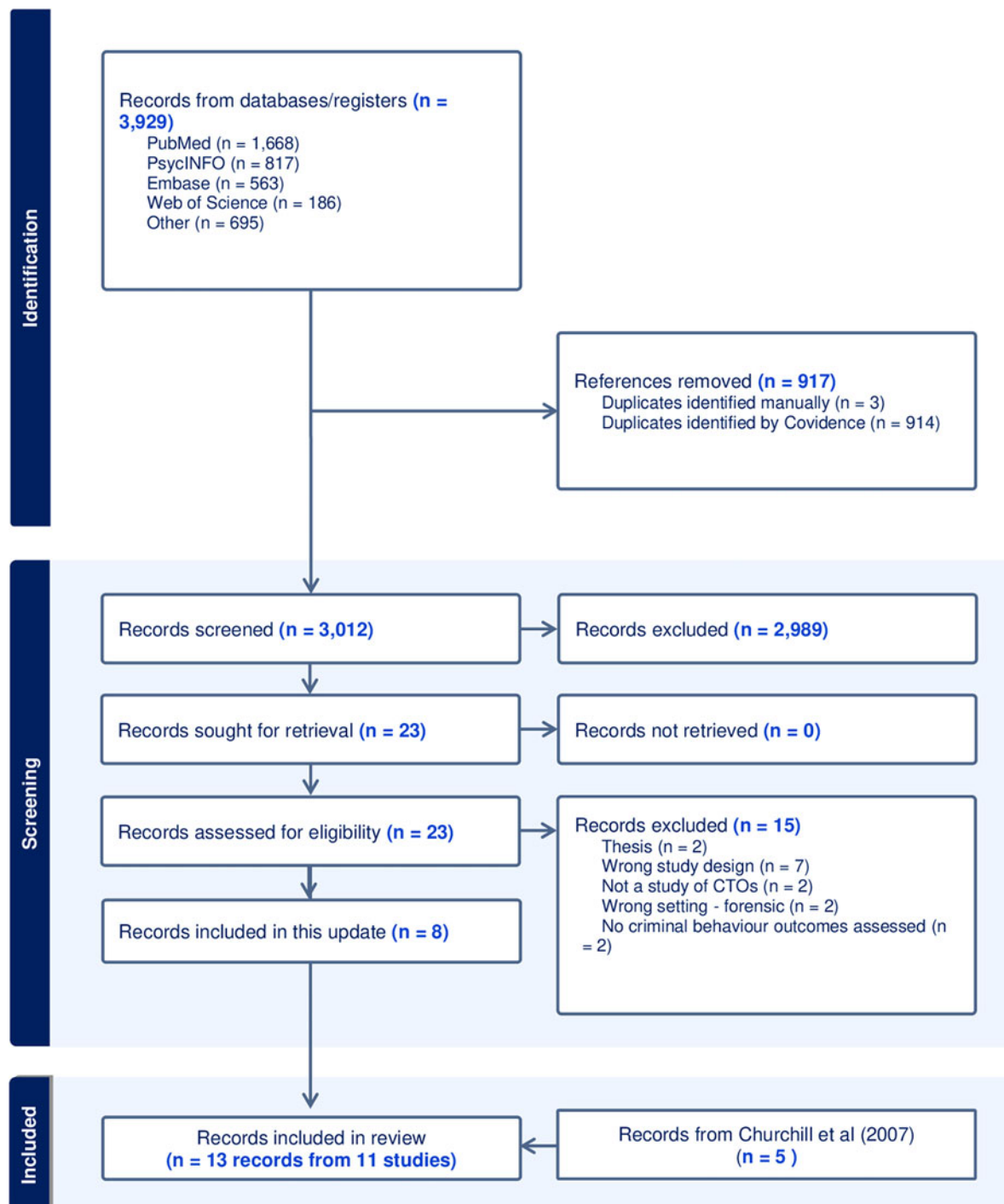
Figure 1. PRISMA diagram.
