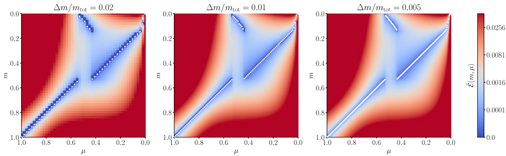
FIGURE 6. The normal form of the cost matrix \tilde{\mathcal{E}}(m, \mu) [see (3.11) for its definition] for the unstable-upwards profile defined by (2.30), for three different choices of the discretisation scale \Delta m . White dots show the optimal assignment.
