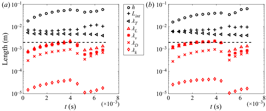
Figure 19. Summary of length scales for the high-amplitude (a), and low-amplitude (b) experiments. Black markers indicate measured scales and red markers indicate scales derived from the outer-scale Reynolds number. The dashed black line indicates four times the Nyquist sampling criterion, which corresponds to the PIV window size and therefore the effective resolution of the diagnostic.
