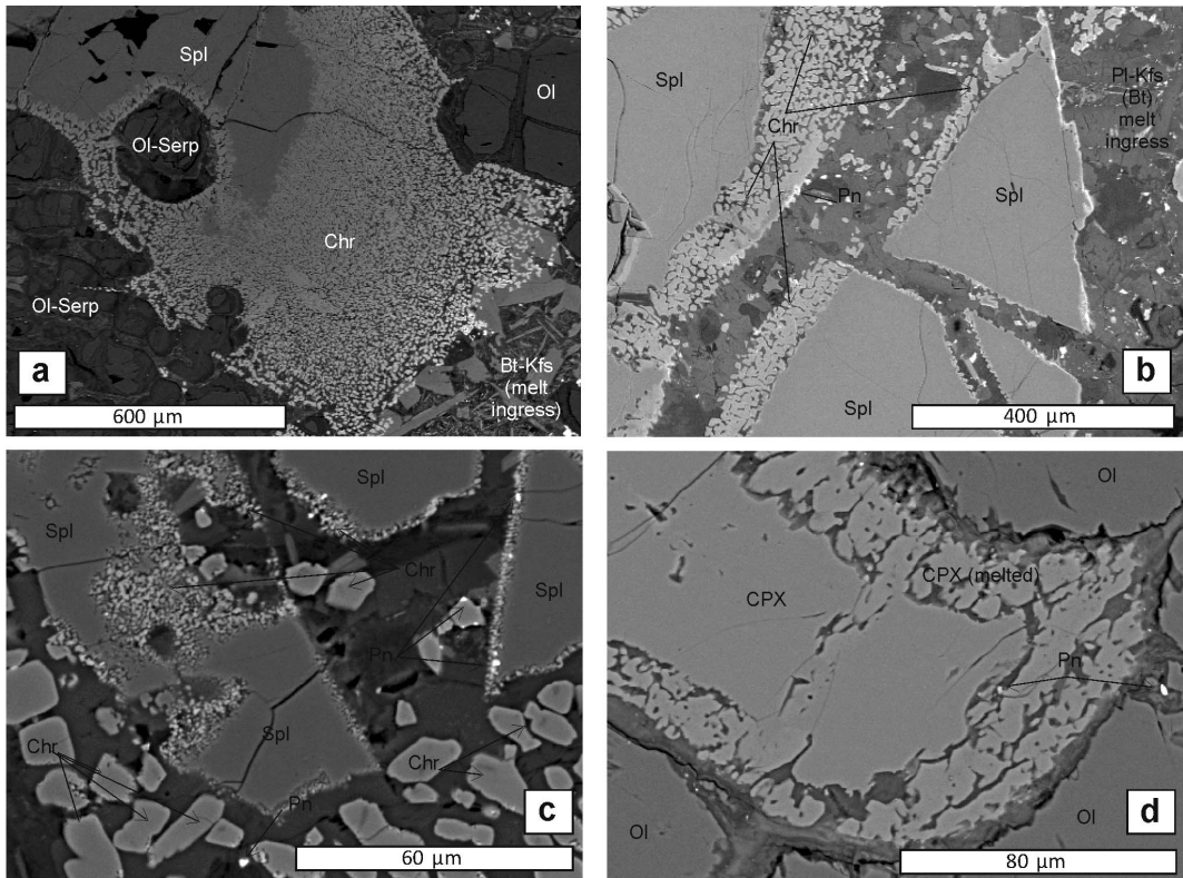
FIG. 4. Strep Com'laidh BSE SEM images. (a) Al-Mg spinel reacting and melting to fine granular chromite at the spinel grain boundary and enclosing granular serpentized olivine. The lower right hand corner of the image shows ingressed orthoclase and biotite-rich melt, possibly from the host dyke entraining the xenolith (sample 4a1). (b) Al-Mg spinel reacting and melting to chromite. Note the tiny \mu\text{m} -scale rounded pentlandite globules associated with spinel-chromite melting (sample 4a1). (c) Similar to (b) with Al-Mg spinel melting at the rim and forming granular chromite. Note the two crystal size populations of chromite: >5\mu\text{m} granular, sub-euhedral chromite crystals vs. \mu\text{m} -scale rounded chromites. Both chromite populations are associated with \mu\text{m} -scale pentlandite globules at crystal margins (sample 4a1). (d) Protogranular clinopyroxene and olivine. Clinopyroxene is melting to form finger-like crystals at its margins. This melt zone is again associated with \mu\text{m} -scale pentlandite globules (sample 4a1). Mineral abbreviations: clinopyroxene (CPX), orthopyroxene (OPX), olivine (Ol), spinel (Spl), chromite (Chr), serpentine (Serp), pentlandite (Pn),
