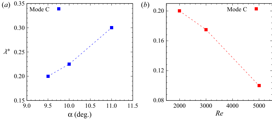
Figure 13. Variation of fastest growing wavelength for mode C (a) with increasing angle of attack \alpha at Re = 2000 , (b) with increasing Reynolds number Re at \alpha = 9.5^\circ .
