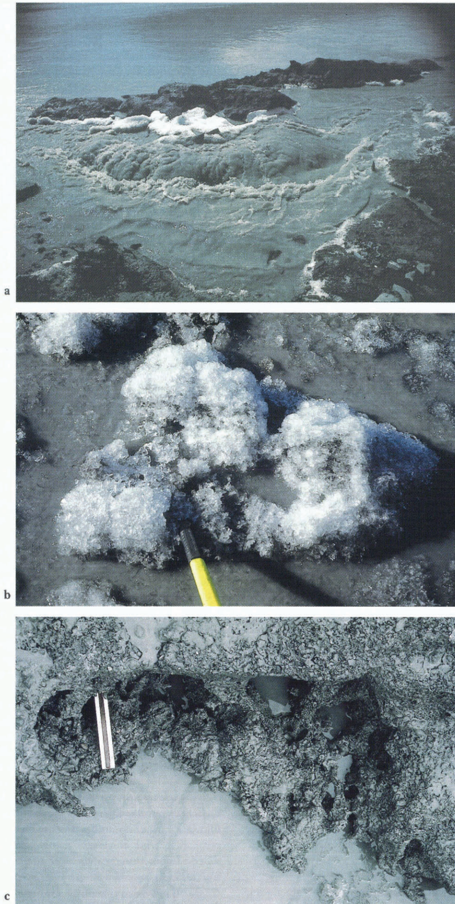
Fig. 4. Examples of vents and anchor and frazil ice in and around vents. (a) Three meter wide vent with raised ( \sim 300 mm) surface of upwelling water. White area is platy anchor ice exposed by the diurnal reduction in discharge; sediment which was discharged from the upwelling lies on other anchor ice surrounding the vent. (b) Aggregate or floc of frazil ice ( \sim 250 mm across) that was captured in a vent after emergence from a subglacial conduit. Tip of ice ax for scale. (c) Debris-laden anchor ice growing into a subglacial conduit exposed at low discharge. Note the upwelling vent water and the clean frazil flocs floating in it.
