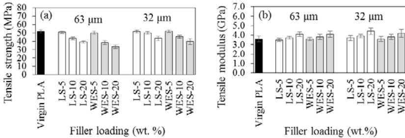
Figure 5. Effect of filler type and loading on the (a) tensile strength and (b) tensile modulus of LS and WES filled PLA composites.
