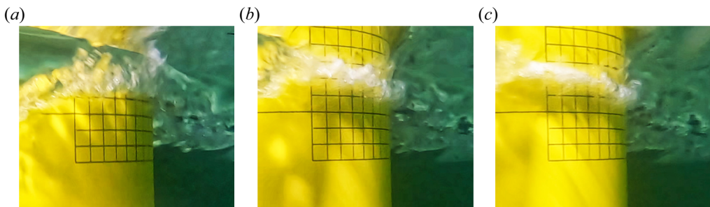
Figure 34. Snapshots of bubble formation for a high aeration wave impact. (a) Breaking wave roller. (b) Closed roller, and bubble formation. (c) Tube shape bubble structures moving towards the sides.
