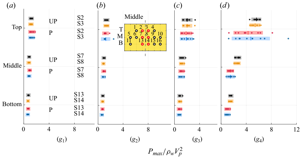
Figure 24. Comparison of pressure variability of the perturbed (P) and unperturbed (UP) tests for all groups using data from the sensors at the middle of the monopile.
