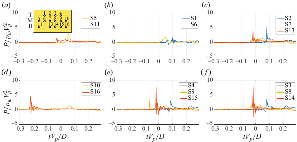
Figure 33. Unperturbed tests event C: pressure oscillations due to the natural frequency excitation and high aeration.
