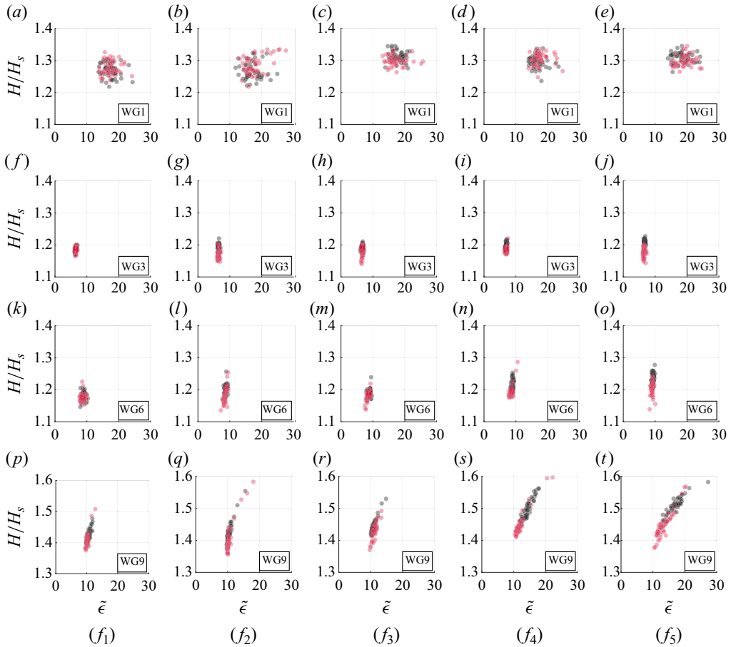
Figure 38. The distribution of maximum wave height and wave slope for the unperturbed and perturbed tests at each focal point: unperturbed shown in black, perturbed in red.
