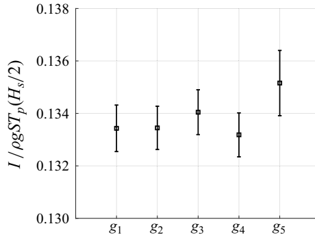
Figure 14. The slamming force impulse variation for each group for the unperturbed tests.
