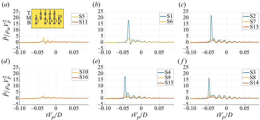
Figure 37. Perturbed tests event E : pressure oscillations due to the natural frequency excitation and high aeration.
