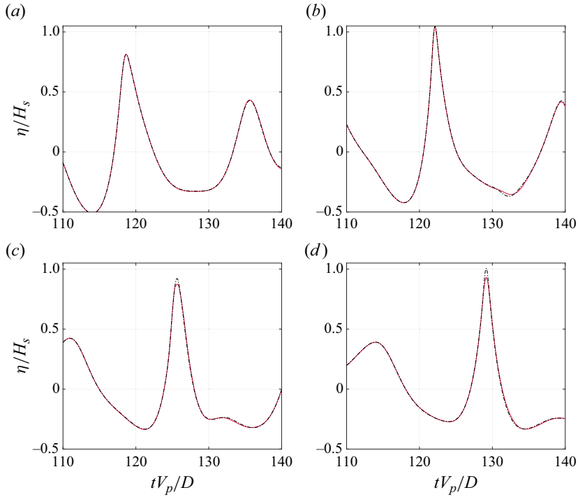
Figure 39. The effect of the wave reflection on the wave height at four different distances from the monopile centre: (a) 3.975 m, (b) 2.975 m, (c) 1.975 m, (d) 0.975 m. No bump indicated with a black dashed line, bump indicated with a red solid line.
