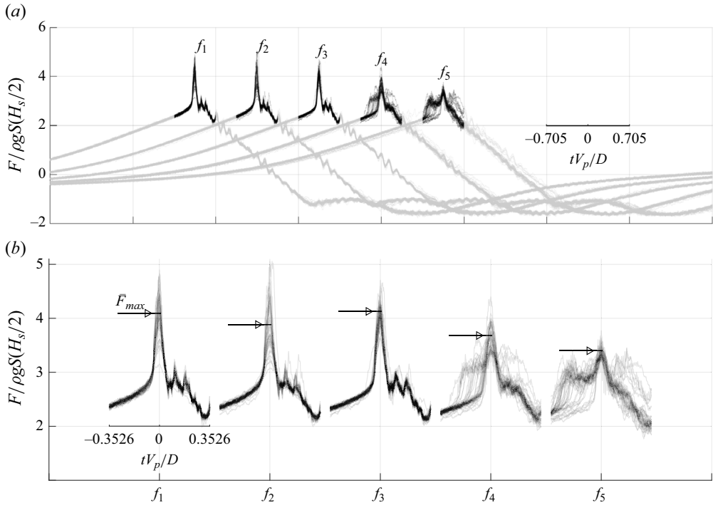
Figure 11. (a) The force time series of 50 test repetitions for five focal points. The slamming part of the force time series that has the highest variability is shown in black, while the rest is shown in grey. (b) The slamming force time series for each focal point. The arrow indicates the mean of the peaks of the slamming forces for each focal point. The time axis is normalized using two parameters: V_p , defined as the ratio of the peak angular velocity to the peak wavenumber, and D , which represents the cylinder diameter.
