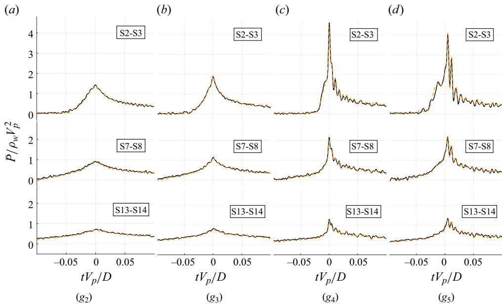
Figure 17. Mean pressure time series for g_2 to g_5 . The time series for each pressure sensor is zero-levelled by the time of the slamming force peak. The left sensor is given by a solid black line; the right sensor is given by a dashed orange line.
