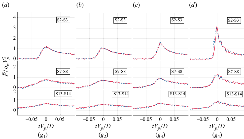
Figure 26. Mean slamming pressure time series of the perturbed tests for g_1 to g_4 . The time series for each pressure sensor is zero-levelled by the time of the slamming force peak. The left sensor is given by a solid red line; the right sensor is given by a blue dashed line.
