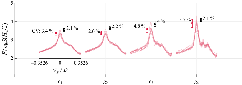
Figure 21. Time series of the slamming force for the regrouped tests. Perturbed is shown in red, unperturbed in black.
