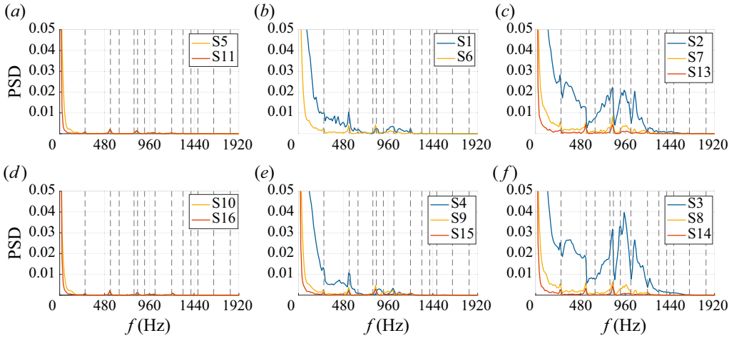
Figure 29. Unperturbed tests event A: pressure oscillations due to the natural frequency excitation.
