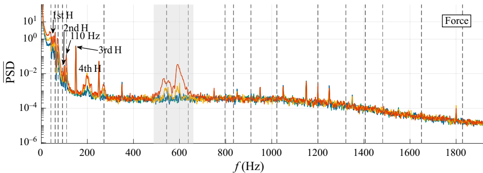
Figure 23. The averaged PSD of slamming force for the perturbed tests for all groups: g_1 in pine green, g_2 in blue, g_3 in yellow, g_4 in red.
