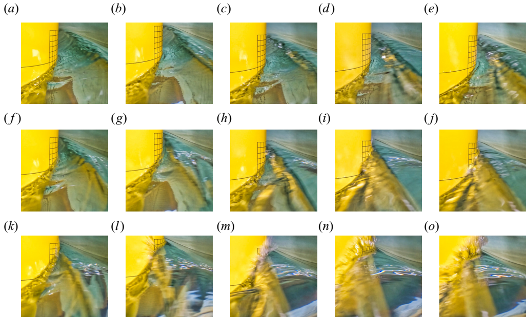
Figure 8. The breaking wave front shapes for f_1 to f_5 for the perturbed waves, where the time difference between each snapshot is 6 \Delta t , with \Delta t = 0.024 s: (a,f,k) f_1 , (b,g,l) f_2 , (c,h,m) f_3 , (d,i,n) f_4 , (e,j,o) f_5 .
