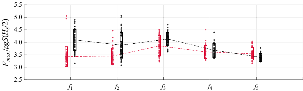
Figure 19. The mean plus/minus one standard deviation of maximum slamming force for all the perturbed and unperturbed tests. The circular markers represent the maximum slamming force value for each test. Perturbed is shown in red, unperturbed in black.
