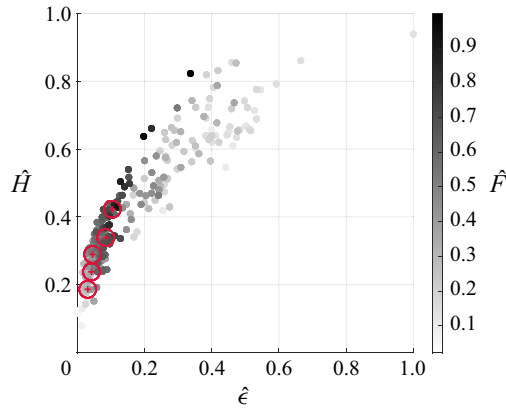
Figure 12. The data illustrate the maximum slamming force recorded in all test cases across different focal points. Five groups of tests are shown, with red circles where efforts were made to minimize wave height and slope. The axes and greyscale have been normalized for consistency.
