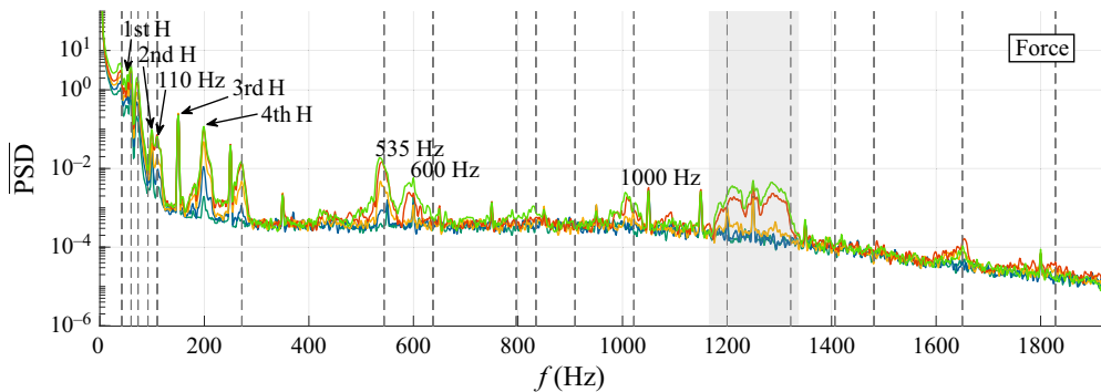
Figure 15. The averaged PSD of slamming force for all groups: g_1 in pine green, g_2 in blue, g_3 in yellow, g_4 in red, and g_5 in lime green. The natural frequencies of the set-up are shown with dashed lines. The electrical current frequency and its harmonics, from 1st H to 4th H, are indicated.
