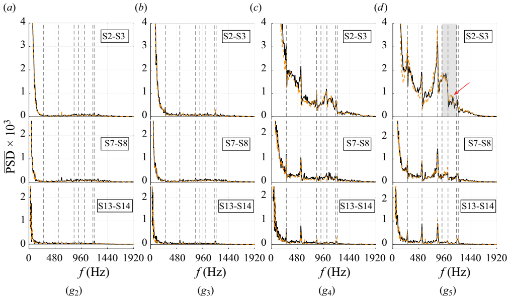
Figure 18. The mean PSD of slamming pressure for g_2 to g_5 . The left sensor is given by a solid black line; the right sensor is given by a dashed orange line.
