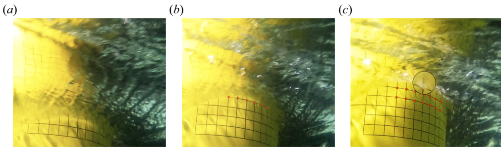
Figure 36. Snapshots of bubble formation for a low-aeration wave impact. (a) Breaking wave roller. (b) Closed roller, and bubble formation. (c) Bubble structures on the pressure sensors.
