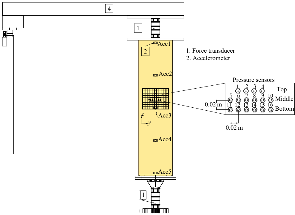
Figure 3. The location of the sixteen pressure sensors, five accelerometers and two force transducers mounted on the monopile.
