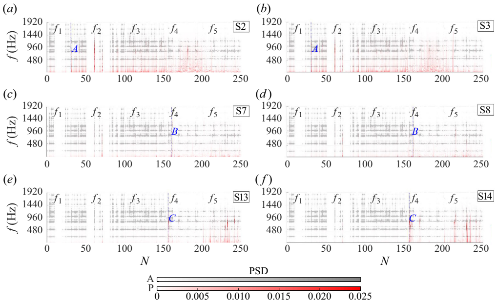
Figure 40. Pressure power spectrum versus accelerometers 2 and 3 power spectra for the unperturbed tests for all focal points.
