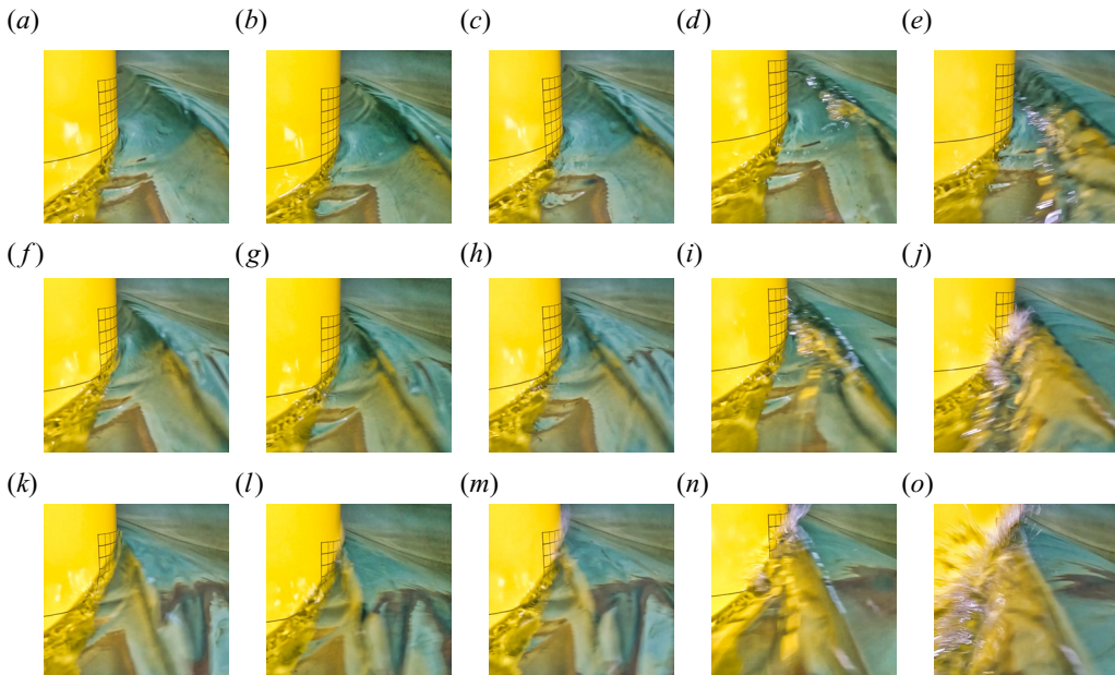
Figure 7. The breaking wave front shapes for f_1 to f_5 for the unperturbed waves, where the time difference between each snapshot is 6 \Delta t , with \Delta t = 0.024 s: (a,f,k) f_1 , (b,g,l) f_2 , (c,h,m) f_3 , (d,i,n) f_4 , (e,j,o) f_5 .
