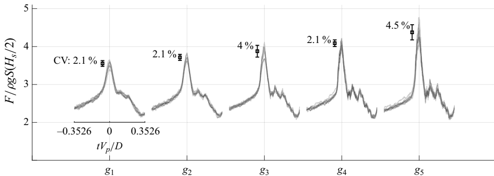
Figure 13. Time series of the slamming force of the regrouped tests.
