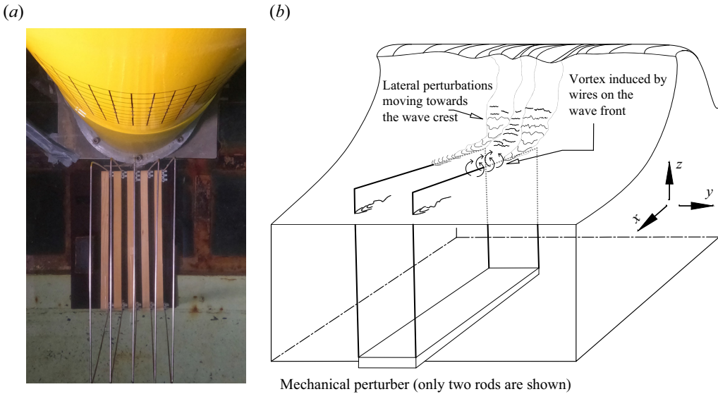
Figure 4. (a) The mechanical perturber with five rods, top view. The support weights are removed. (b) Schematic of the perturber interacting with the incoming wave.
