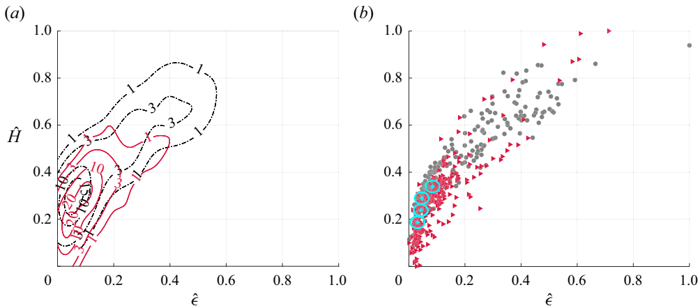
Figure 20. (a) Probability density estimation of the unperturbed and perturbed tests: unperturbed with a black dashed line, perturbed with a solid red line. (b) Scatter plot of the normalized wave height and wave slope for the unperturbed and perturbed tests. The circles show the location of each group; unperturbed shown with grey dots, perturbed with red triangles.
