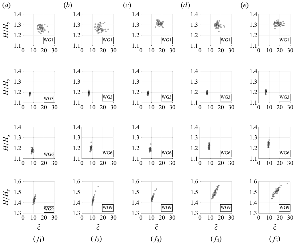
Figure 10. The distribution of the maximum wave height and wave slope for all the unperturbed waves in f_1 to f_5 .
