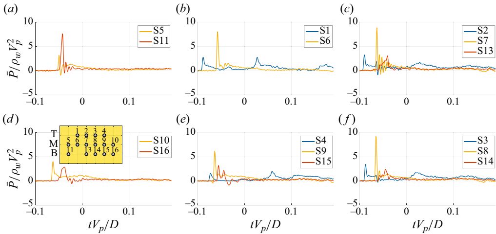
Figure 31. Unperturbed tests event B : pressure oscillations due to the natural frequency excitation and medium aeration.
