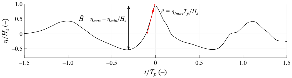
Figure 9. Definitions of the wave height and the wave slope. The horizontal and vertical axes are, respectively, non-dimensionalized by T_p and H_s .
