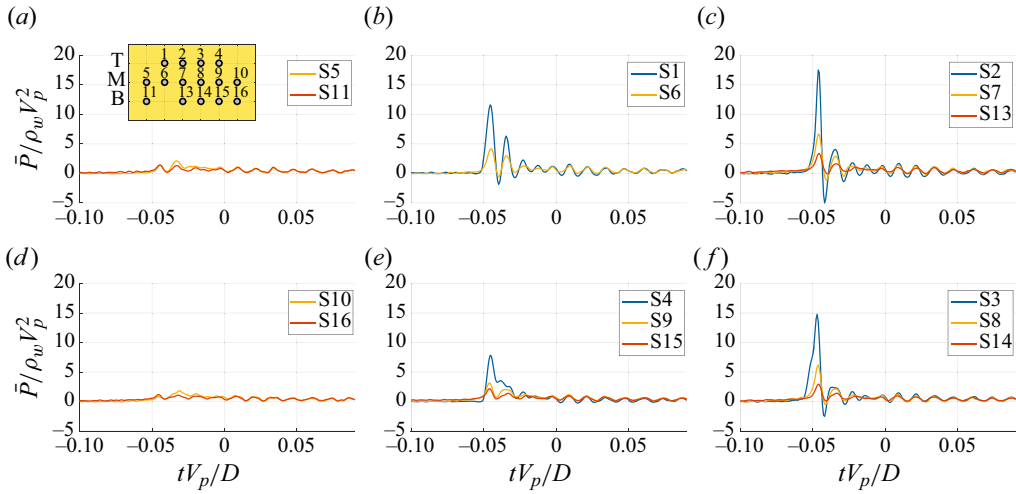
Figure 35. Perturbed tests event D : pressure oscillations due to the natural frequency excitation and high aeration.
