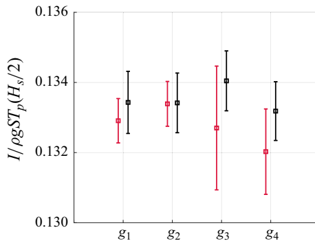
Figure 22. The slamming force impulse variation for each group of tests. Perturbed is shown in red, unperturbed in black.
