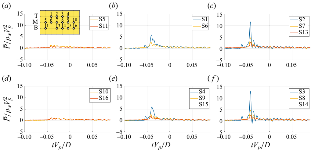
Figure 28. Unperturbed tests event A : pressure oscillations due to the natural frequency excitation and low aeration.
