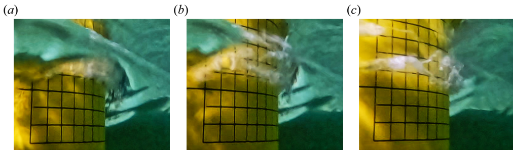
Figure 32. Event B : snapshots of bubble formation for a medium aeration wave impact. (a) Water and gas mixture by jets shoots up inside the breaking wave roller. (b) Closed roller, and bubble formation. (c) Tube shape bubbles on the pressure sensors area.
