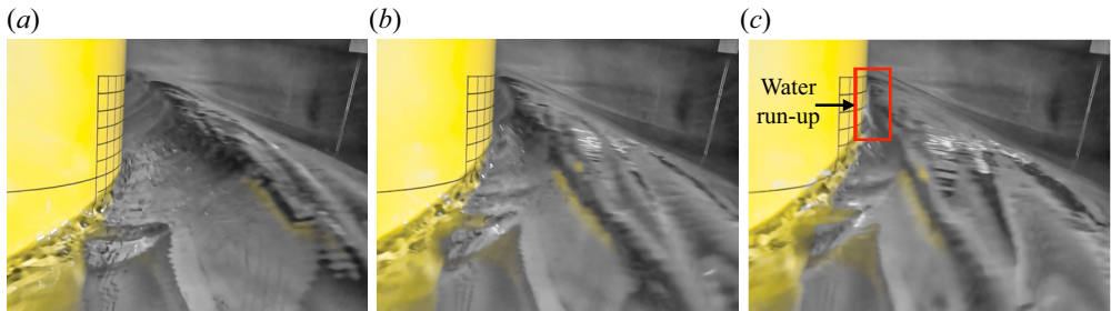
Figure 25. Snapshots of the slosh impact for a perturbed test: (a) t_0 , (b) t_0 + 1 \Delta t , (c) t_0 + 2 \Delta t .
