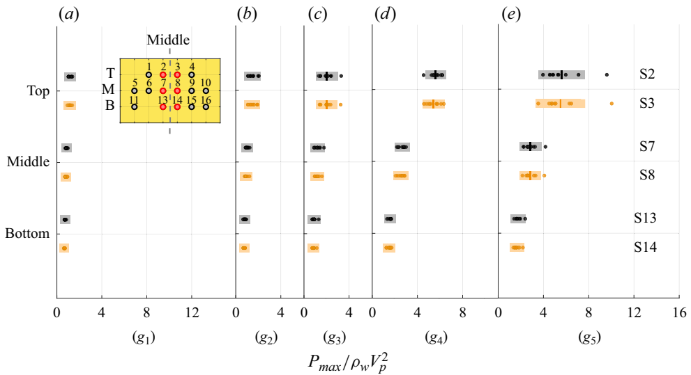
Figure 16. Distribution and variation of the slamming pressure at the area in the middle of the monopile. Sensors to the left of the middle axis are shown in black; sensors to the right of the middle axis are shown in orange.
