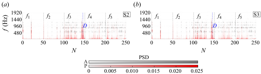
Figure 41. Pressure power spectrum versus accelerometers 2 and 3 power spectra for the perturbed tests for all focal points.
