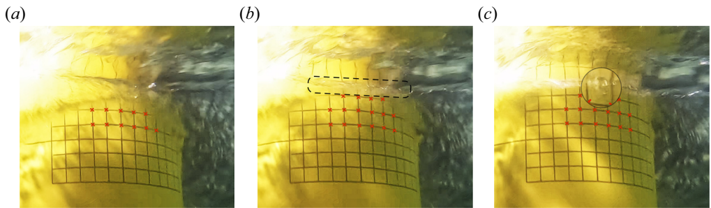
Figure 30. Event A: snapshots of small-bubble formation for a low-aeration wave impact. Note that the bubble is magnified. (a) Breaking wave roller. (b) Closed roller, and bubble formation. (c) Bubbles transitioning towards the water surface.
