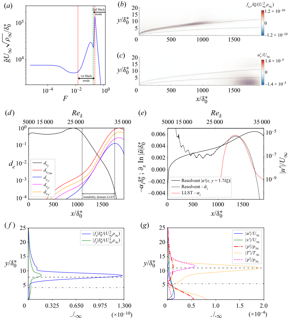
Figure 3. (a) Optimal resolvent gain as a function of the dimensionless frequency F . According to LLST, red and green dashed areas represent the unstable range of first and second Mack modes, respectively. The region where both modes are unstable corresponds to an area where the first mode is unstable over a tiny distance. (b) Real part of the streamwise component of the optimal forcing and (c) its associated streamwise velocity response, at F = 0.237 . (d) Evolution at F = 0.237 of the forcing density and the different contributions to the Chu energy density normalized by their maximum values. The positions of branches I and II from LLST are symbolized by vertical dashed lines. (e) Comparison of -\alpha_i and -\tilde{\alpha}_i at F = 0.237 . (f) Profiles of the optimal forcing components at x = 867.2\delta_0^* , and (g) response at x = 1766.7\delta_0^* , at F = 0.237 . The black dashed and dashed-dotted lines in (b), (c), (f) and (g) represent respectively the generalized inflection point position and the limit of the region of supersonic instabilities ( \hat{M} > 1 below this line).
