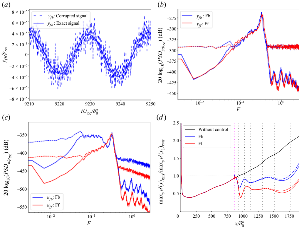
Figure 12. In all plots, feedback and feedforward designs are represented by blue and red lines, respectively. Controlled systems with ideal and noisy estimation sensors are represented by solid and dashed lines, respectively. (a) Short sequence of y_{fb} corrupted by 50% of the r.m.s. value without control of y_{fb} . Comparison of the evolution of PSD_y (b), PSD_u (c) and \max_y u'_{rms} (d) for the controlled systems with ideal and noisy estimation sensors. The details for (d) are the same as in figure 8(c).
